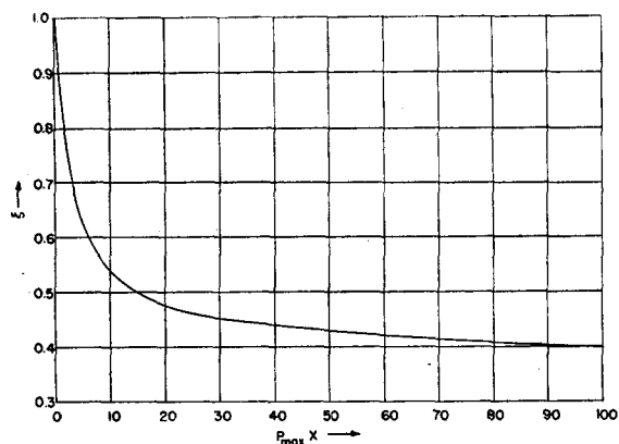
FIG. 16. The quantity \xi as a function of P_{\max}X .
