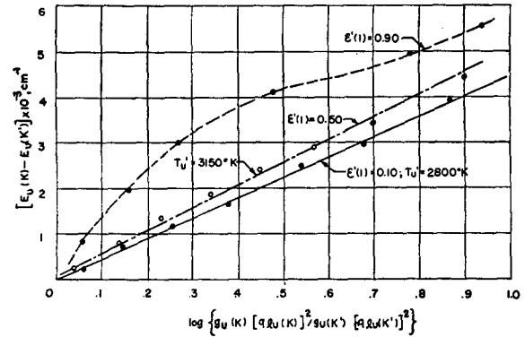
FIG. 8. Plot of [E_u(K) - E_u(K')] \times [q_{lu}(K)]^2/g_u(K') \times [q_{lu}(K')]^2 for lines with equal peak intensities at 3000°K as a function of \epsilon'(1) for the P_1 branch, (0,0) band, {}^2\Sigma \rightarrow {}^2\Pi transitions of OH.
