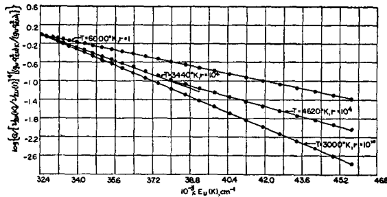
FIG. 10. Conventional plots and apparent temperatures for various bimodal distributions of OH.
