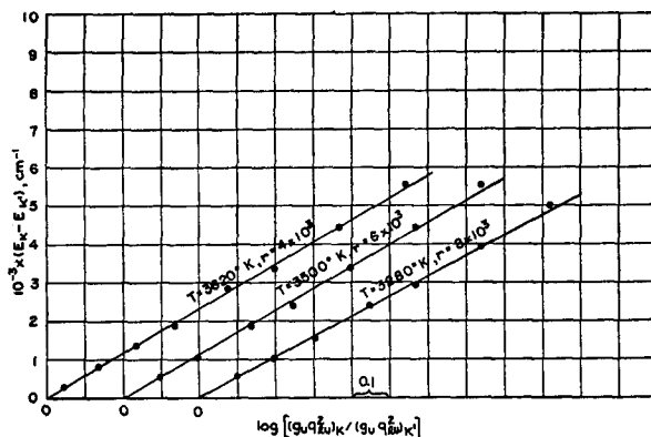
FIG. 13. Isointensity plots and apparent temperatures for r = 4 \times 10^2 , 6 \times 10^2 , and 8 \times 10^2 .
