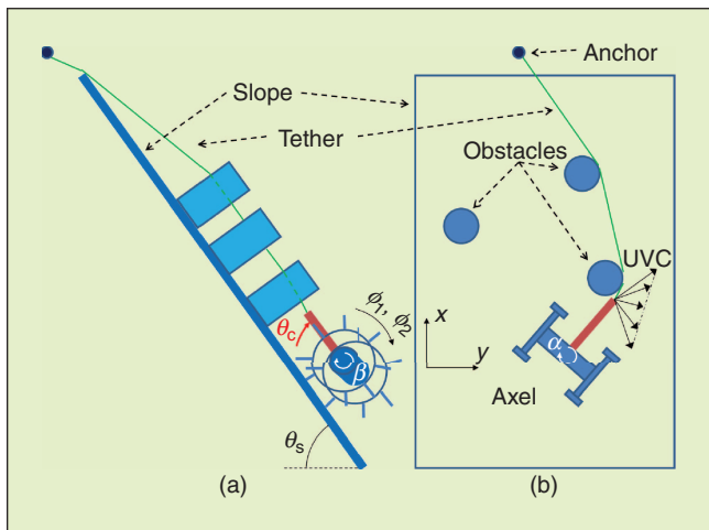
Figure 12. Schematic diagram of Axel on slope with obstacles: (a) side and (b) frontal views.
