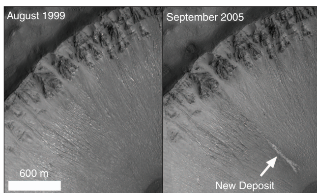
Figure 1. Photos from the Mars Global Surveyor orbiter camera showing recent flows in a crater of the Centauri Montes region. (Courtesy of NASA's Mars Global Surveyor.)
