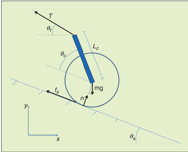
Figure 7. Two-dimensional free-body diagram of tethered Axel on a slope.
