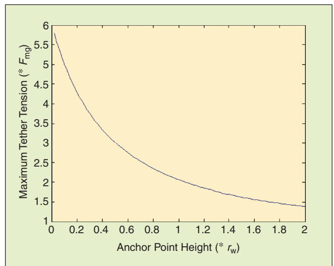
Figure 11. Maximum tether tension versus anchor point height for geometry of Figure 9 ( d = 2r_w and \mu = 0.25 ).
