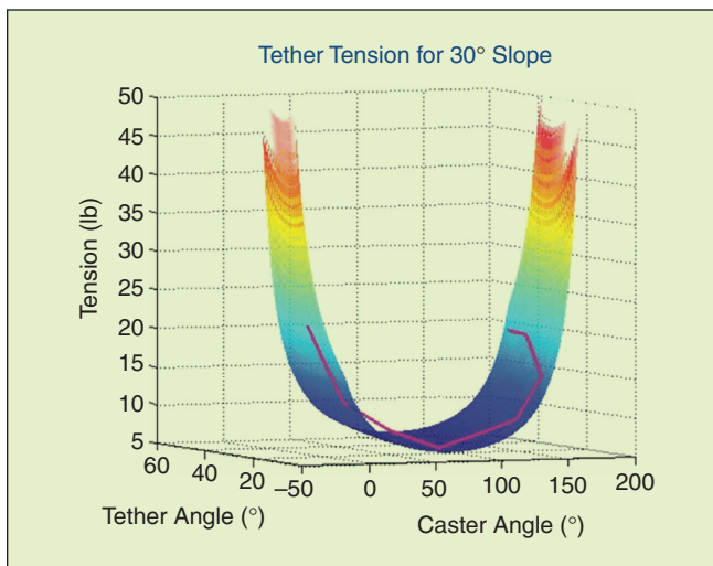
Figure 8. Predicted tether tension versus tether and caster angle for 30° slope. Measured tension, represented by the purple line, is overlaid on the theoretical prediction.
