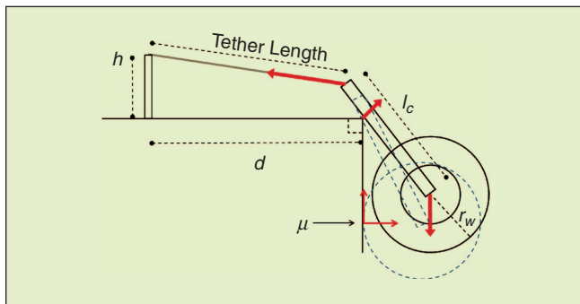
Figure 9. Free-body diagram of Axel ascending over a ledge. Initially, wheels are in contact with the wall, but separate from the wall as winching progresses.
