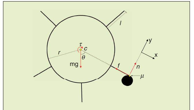
Figure 6. Force diagram of a paddle wheel as it encounters an obstacle and just as it leaves the ground.
