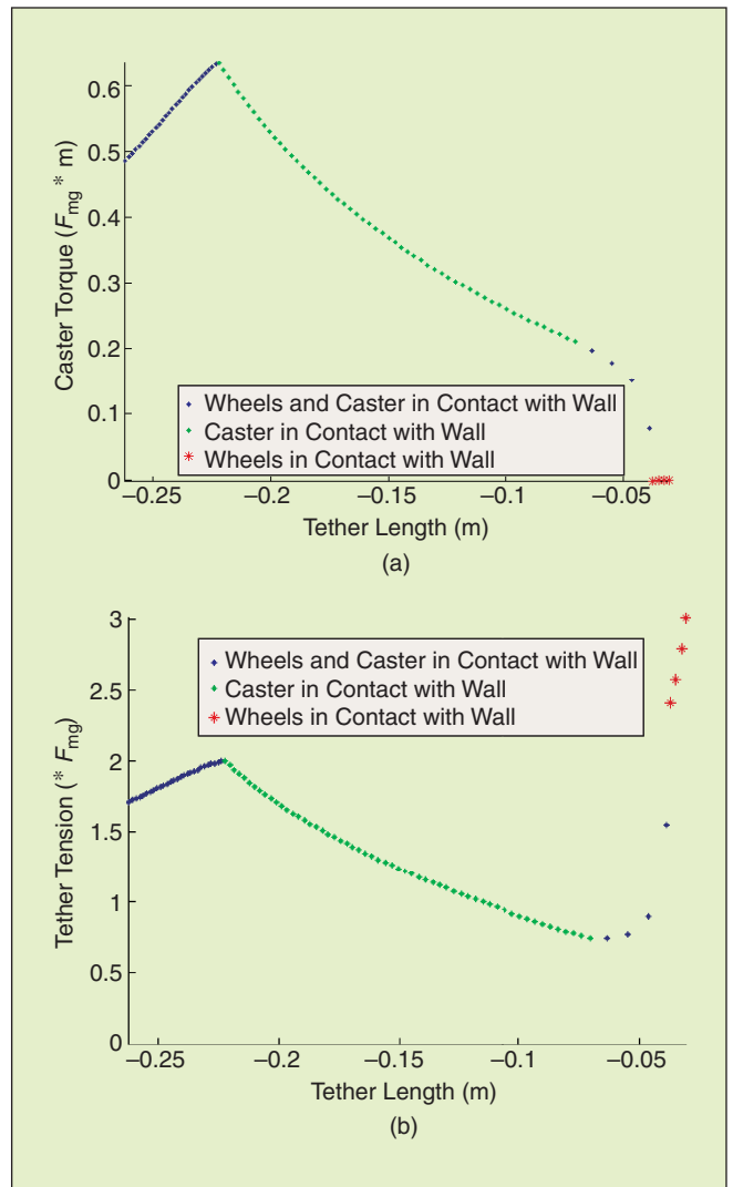
Figure 10. (a) Caster motor torque and (b) tether tension versus tether length for geometry of Figure 9 ( d = 2r_w , h = 0.5r_w , and \mu = 0.25 ).
