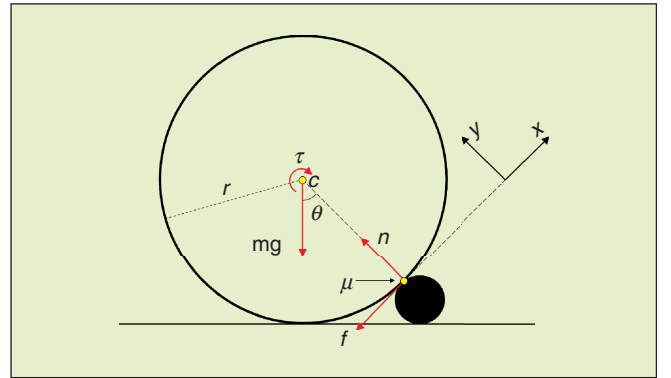
Figure 5. Free-body diagram of a wheel traveling over a rock just as it loses contact with the ground.
