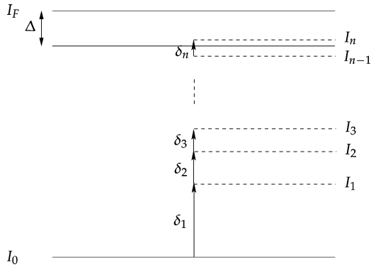
Fig. 12. A pictorial illustration of the modeled programming sequence. On the left side are the initial level I_0 , the target level I_F and the tolerance parameter \Delta . In the middle is a sequence of exponentially distributed level increments \delta_1, \delta_2, \dots, \delta_n resulting from the programming algorithm. On the right side are the instantaneous levels I_i until the process terminates at I_n .
