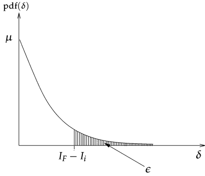
Fig. 11. Choice of a programming distribution based on the specified probability of overprogramming. For starting level I_i and target level I_F the parameter \mu of the exponential distribution is chosen such that the marked area under the probability density function graph equals \epsilon (the specified probability of overprogramming).
