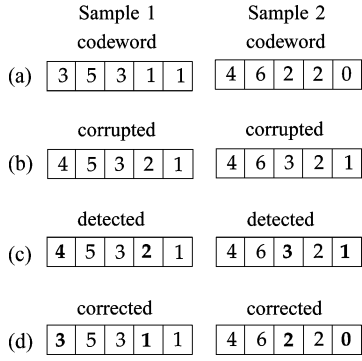
Fig. 1. Example of correcting asymmetric limited-magnitude errors.
