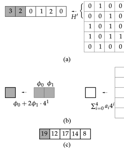
Fig. 6. Encoding of a systematic code with t = 1 and \ell = 3 .
