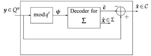
Fig. 2. Decoding asymmetric \ell -limited-magnitude error-correcting codes.
