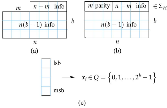
Fig. 3. Encoding Procedure for \mathcal{C}_H .
