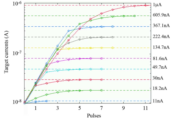
Fig. 10. Performance of a flash adaptive program sequence [3]. The circles on each curve describe the results of an iterative programming algorithm for a given target value.
