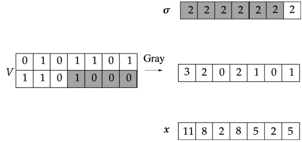
Fig. 8. Example of a code for asymmetric and symmetric limited-magnitude errors. From top to bottom: a codeword \sigma of the ternary repetition code; a binary Hamming codeword arranged into a 2 \times 7 array and its Gray mapping; the final codeword \mathbf{x} obtained by combining \sigma and V .
