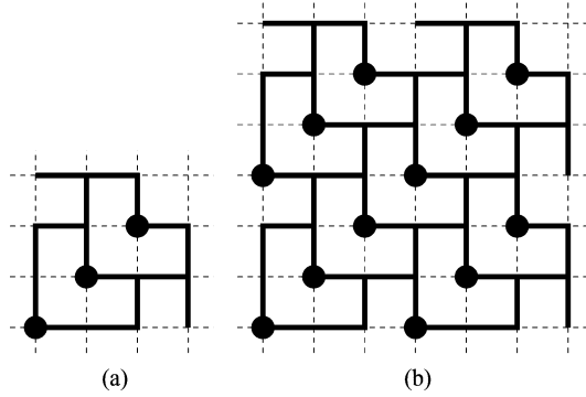
Fig. 4. In Example 2, the tilings induced by (a) the code \Sigma , and (b) the code \mathcal{C} .
