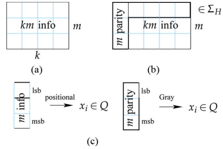
Fig. 5. Encoding procedure for a systematic code.
