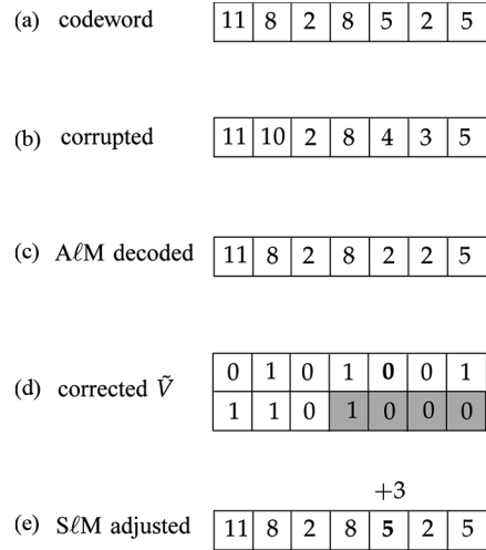
Fig. 9. Example of decoding asymmetric and symmetric limited-magnitude errors. (a) Codeword. (b) Codeword corrupted by asymmetric and symmetric limited-magnitude errors. (c) First decoding step: correction of asymmetric limited-magnitude (ALM) errors. (d) Resulting corrected codeword \tilde{V} is decoded using a Hamming decoder. (e) Adjusting the miscorrection of the symmetric error found in the previous step.
