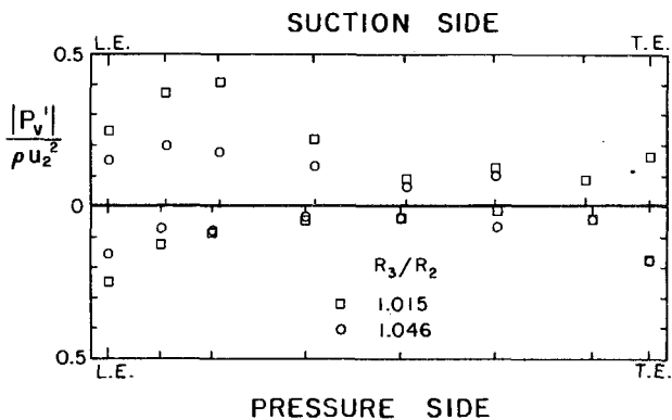
Fig. 6 Averaged instantaneous vane pressure measurements for Impeller R at vane centerline. RPM=1800, d=.12 , R_3/R_2=1.015 and 1.046
