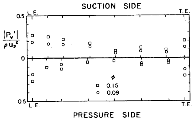
Fig. 7. Averaged instantaneous vane pressure measurements for Impeller R at vane centerline. RPM=1800, \phi=.15 and .09 , R_3/R_2=1.046
