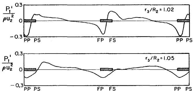
Fig. 5a and 5b. Averaged instantaneous total pressure measurements for Impeller R at centerline of Volute D for r_3/R_2=1.02 (top) and r_3/R_2=1.05 (bottom). RPM = 1200, d=.12 , the cross-hatching indicates the blade trailing edge. FP=full blade pressure side, FS=full blade suction side, PP=partial blade pressure side, PS=partial blade suction side
