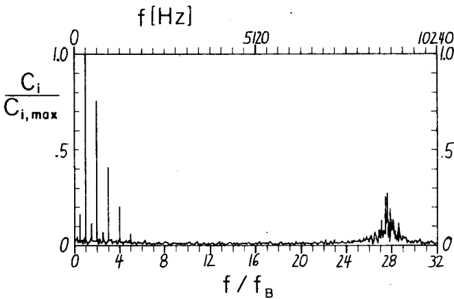
Fig. 3. Magnitude of normalized Fourier coefficients for instantaneous vane pressure measurements at suction side tap 1 (rpm=2400, \phi=.15 , R_3/R_2 = 1.046 )
