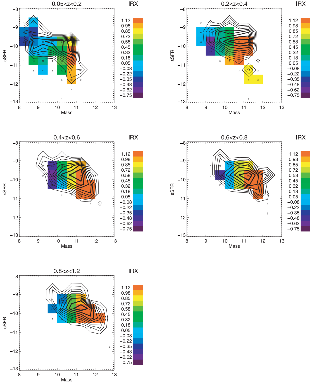
FIG. 6.—Volume-corrected, bivariate mass-SSFR distribution weighted by the SFR: \text{SFR} \times \phi(\mathcal{M}, \text{SSFR}) . Contours are equally spaced in (\log \text{SFR})\phi [ \mathcal{M}_{\odot} \text{yr}^{-1} \text{Mpc}^{-3} ], with 10 divisions over -4 < (\log \text{SFR})\phi < -1 . Colors give the IRX, which is the log of the FUV-to-FIR luminosity ratio.
