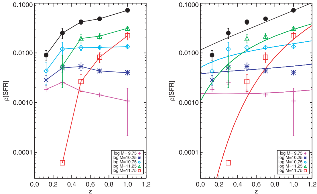
FIG. 18.—Star formation rate density [ \text{M}_\odot \text{yr}^{-1} \text{Mpc}^{-3} ] vs. redshift derived assuming a nonevolving mass function. Error bars are based on bootstrapping but do not include cosmic variance, which adds a relative error of 0.37 to all the measurements. Left : Density in each mass bin, with 9.5 < \log \mathcal{M} < 10.0 (purple), 10.0 < \log \mathcal{M} < 10.5 (blue), 10.5 < \log \mathcal{M} < 11.0 (cyan), 11.0 < \log \mathcal{M} < 11.5 (green), 11.5 < \log \mathcal{M} < 12.0 (red), and total (black). Right : Compared with a simple IRX-SSFR model, for each mass bin (colors are as in the left panel) and for the total (black).
