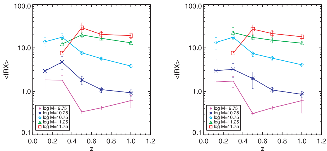
FIG. 8.—Average IRX ( \langle \text{IRX} \rangle ; linear version plotted on a logarithmic scale) vs. redshift in each mass bin. Left , numerical average; right , SFR-weighted average. Errors are derived from bootstrapping.
