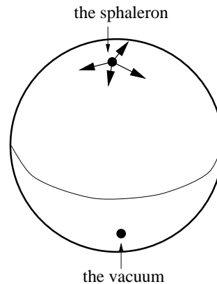
Figure 4: Non-contractible 2n - 1 -sphere in the configuration space and the corresponding n sphaleron configuration.
