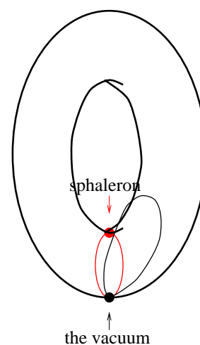
Figure 3: The topological argument tying the existence of a non-contractible loop in the configuration space with the existence of a static solution with one negative eigenvalue (the sphaleron). The vertical axis corresponds to the energy.
