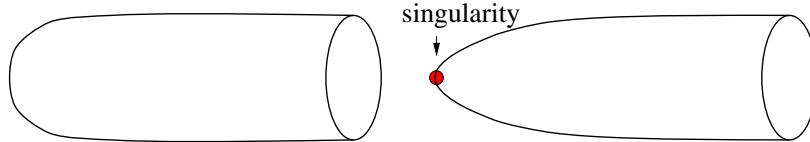
Figure 2: Two supergravity solutions: (a) The euclidean Schwarzschild black hole in eleven dimensions; (b) the type-IIA D-instanton.
