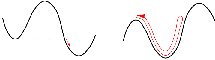
Figure 1: False vacuum decay and the euclidean instanton (the “bounce”) with one negative eigenvalue that dominates the path integral. (a) Tunnelling from the false vacuum. (b) The Euclidean bounce solution.
