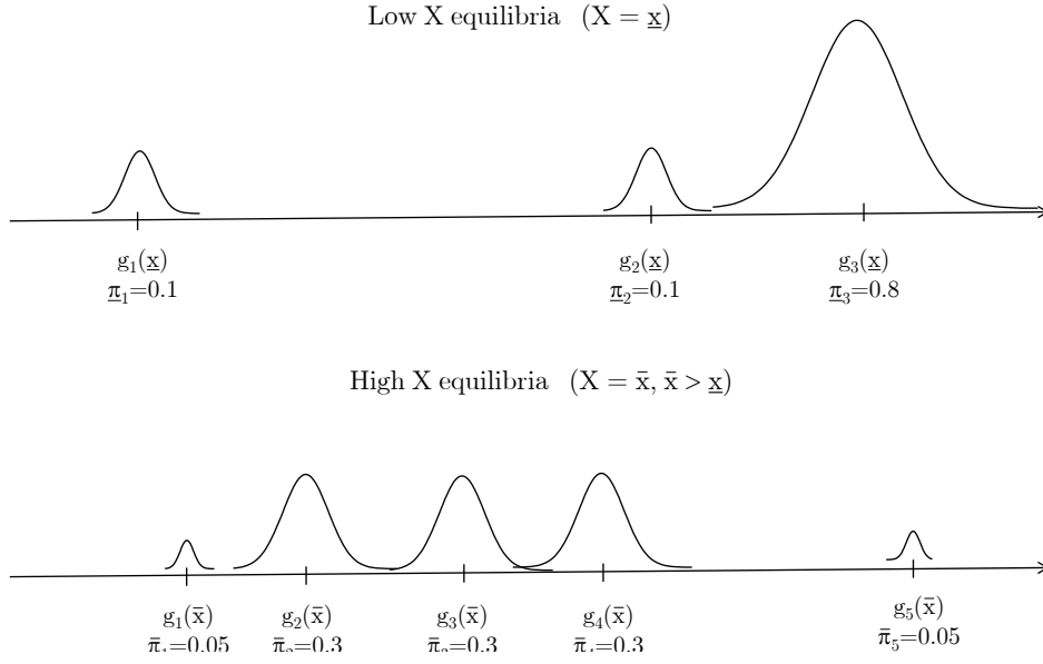
FIGURE 2. Equilibrium distributions.
