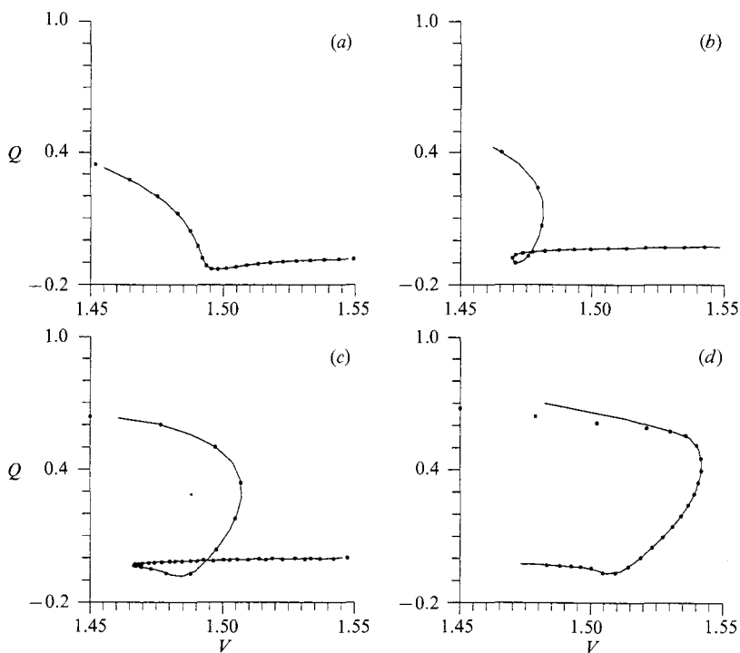
FIGURE 17. Solution sensitivity to pipe length, Z , using \bullet , Z = 30 and —, Z = 60 with \alpha = 0.05 and (a) Re = 250 (b) Re = 500 (c) Re = 1000 (d) Re = 2000 .
