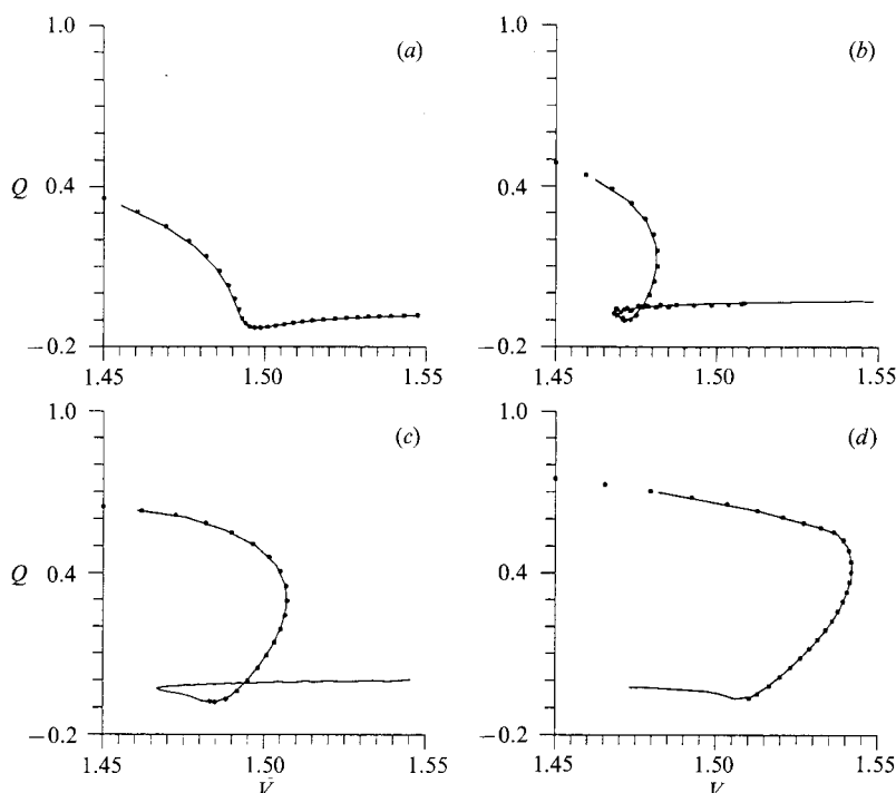
FIGURE 8. Solution sensitivity to axial node spacing, \Delta_z , using \bullet , I = 151 and —, I = 301 with \alpha = 0.05 , J = 27 , and (a) Re = 250 (b) Re = 500 (c) Re = 1000 (d) Re = 2000 .
