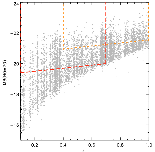
Fig. 1. B -band rest frame absolute magnitudes as a function of redshift for galaxies of the 10k-sample residing in the central area of the zCOSMOS field, in the redshift range considered in this paper. Two time-evolving luminosity volume limits are shown with dashed lines: the red long-dashed line represents the fainter limit ( M_B = -19.3 - z ), for which we are complete up to z = 0.7 , and the orange short-dashed line is the limit M_B = -20.5 - z , for which we are complete up to z = 1.0 but for which we have enough galaxies only for z \geq 0.4 .
