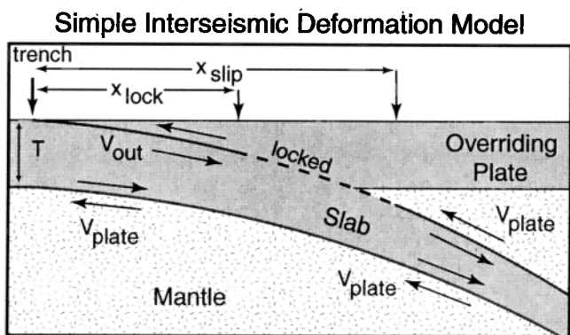
Figure 4. Sketch showing the parameters of an idealized model of interseismic deformation at a subduction zone.
