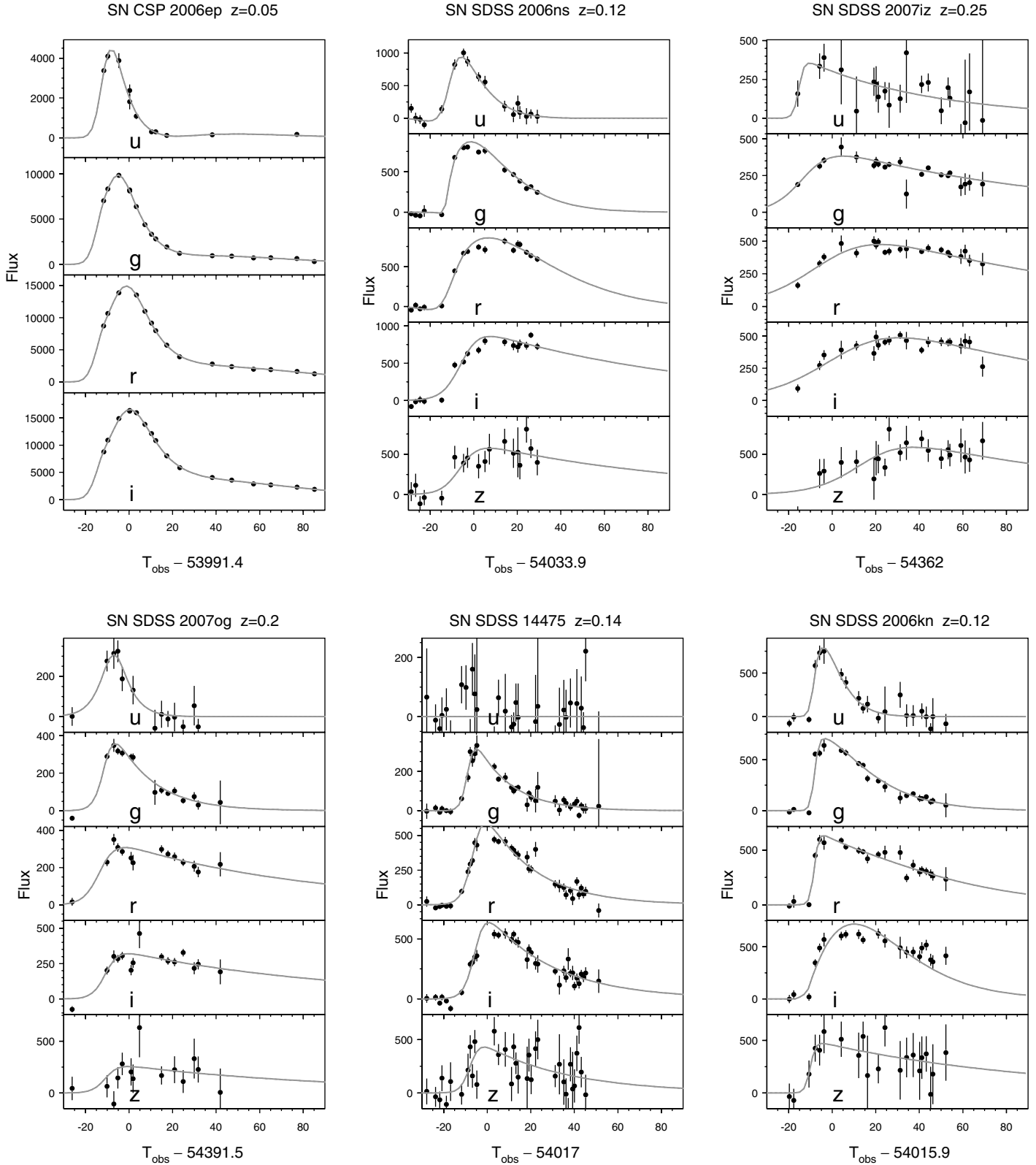
FIG. 1.—Spectroscopically confirmed non-Ia SNe data (black dots) resulting in the most misidentified non-Ia in the SNPhotCC. The smoothing function in Eq. (1) is shown by the curve. The SN name and redshift are listed above each set of light curves. The filter is labeled in each panel. See the electronic edition of the PASP for a color version of this figure.
