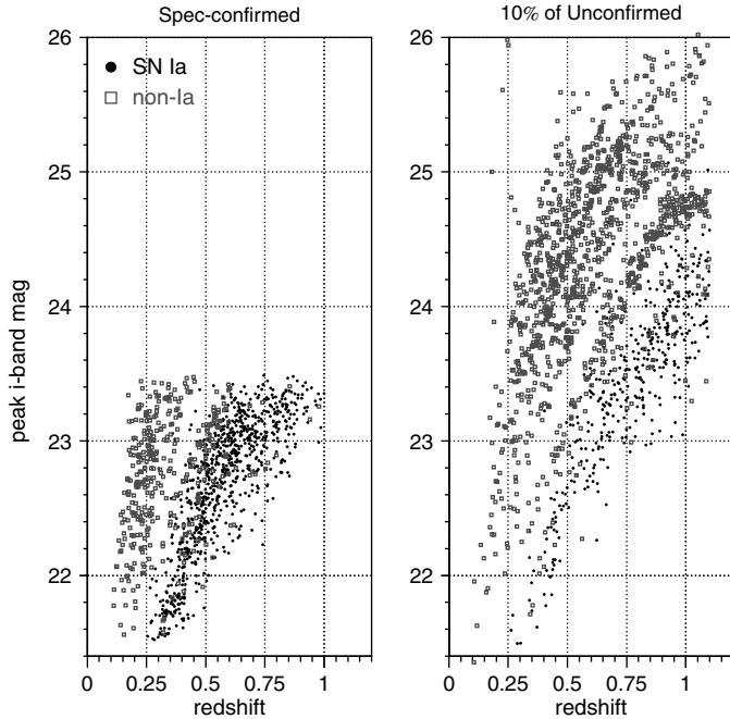
FIG. 2.—For SNe with r > 21.5 at peak brightness, peak i -band magnitude vs. redshift for the spectroscopically confirmed subset ( left ) and for 10% of the unconfirmed sample ( right ). The SNe Ia are shown by filled circles; the non-Ia SNe by open squares. The dashed grid lines are shown to guide the eye. See the electronic edition of the PASP for a color version of this figure.
