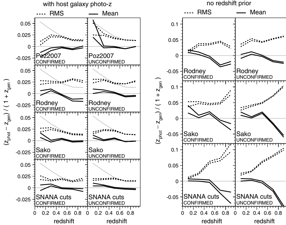
FIG. 7.—Photo- z residuals (z_{\text{phot}} - z_{\text{gen}})/(1 + z_{\text{gen}}) vs. redshift for the SNPhotCC/HOSTZ ( left ) and SNPhotCC/noHOSTZ ( right ). The mean residual is shown by solid curves, and the rms by the dashed curves. The dotted curves (same in each SNPhotCC/HOSTZ panel) show the rms for the host-galaxy photo- z . Note that the vertical scales are different for the left and right plots. See the electronic edition of the PASP for a color version of this figure.
