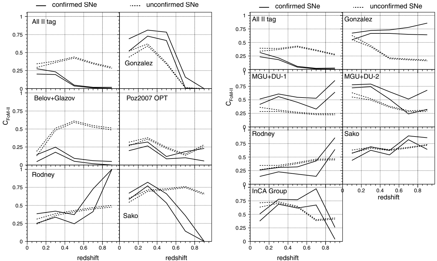
FIG. 6.—Figure of merit versus redshift for type II classifications from the SNPhotCC/HOSTZ ( left ) and from the SNPhotCC/noHOSTZ ( right ). The first panel, labeled “All II tag,” is an arbitrary reference in which every SN has been tagged as a type II, thereby ensuring 100% efficiency. The solid curves show \pm 1\sigma_{\text{stat}} values for the spectroscopically confirmed subset, and the dashed curves are for the unconfirmed SNe.
