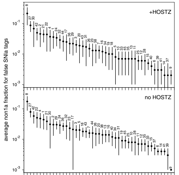
FIG. 3.—Among all generated non-Ia SNe that were falsely tagged as an SN Ia, the average fraction of each non-Ia template is shown. Error bars reflect the rms dispersion among the submissions. The SNPhotCC index shown above each data point is translated in Table 2.
