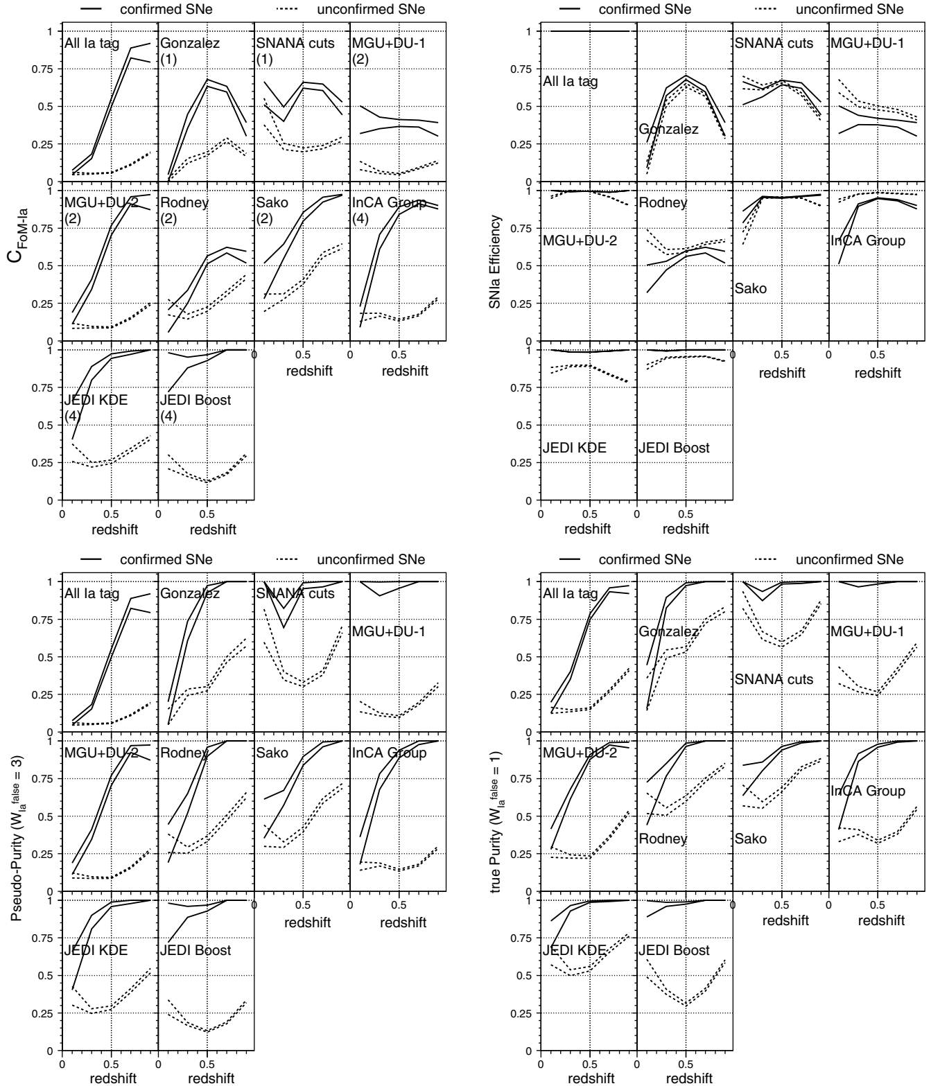
FIG. 5.—For each participant in the SNPhotCC/noHOSTZ, results vs. redshift are shown for C_{\text{FoM-Ia}} , \epsilon_{\text{spec}} , pseudopurity ( PP_{\text{Ia}} ), and the true purity ( PP_{\text{Ia}} with W_{\text{Ia}}^{\text{false}} = 1 ). The first panel, labeled “All Ia tag,” is an arbitrary reference in which every SN has been tagged as an SN Ia, thereby ensuring 100% efficiency. The solid curves show \pm 1\sigma_{\text{stat}} values for the spectroscopically confirmed subset, and the dashed curves are for the unconfirmed SNe. Entries are arranged by method categories 1–4 (§ 3) as indicated in parentheses under the participant names in the first panel.
