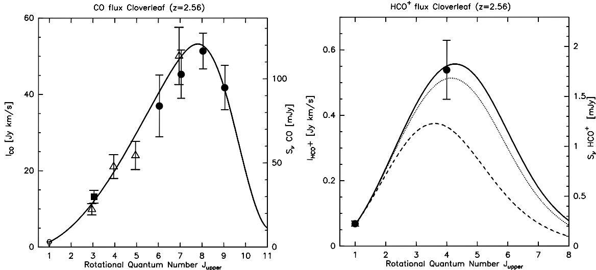
FIG. 3.— CO ( left ) and HCO + ( right ) excitation ladders (points) and LVG models (lines) for the Cloverleaf. Left : The CO data (circle: Tsuboi et al. 1999; triangles: Barvainis et al. 1997; filled square: Weiß et al. 2003; filled circles: Bradford et al. 2009) are fit well by a gas component with a kinetic temperature of T_{kin}=50 K and a gas density of \rho_{gas}=10^{4.5} cm -3 . Right : The HCO + data are fit well by a dense gas component with T_{kin}=50 K and \rho_{gas}=10^{4.8} cm -3 (i.e., 2\times\rho_{gas} of CO; solid line). For comparison, the dashed line shows a model with the same \rho_{gas} as in the CO model, and a 10^{0.5}\times higher HCO + abundance as in the other models. All models are scaled to the same HCO + ( J=1\rightarrow 0 ) flux.
