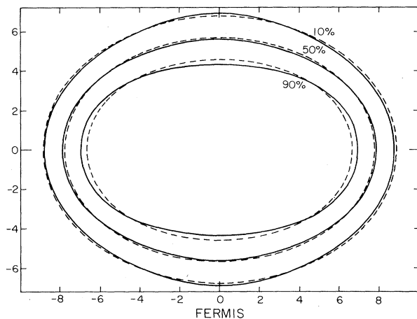
FIG. 1. Contour plots of the angular distribution \rho(r, \theta) of ^{165}\text{Ho} , Eq. (4), showing a cut through the poles. The dashed contours correspond to the best-fit parameters assuming \eta=0 . The solid curves correspond to the fit where the skin-thickness deformation parameter \eta was allowed to vary. Each set of three curves denotes the 90%, 50%, and 10% profiles relative to the central density.
