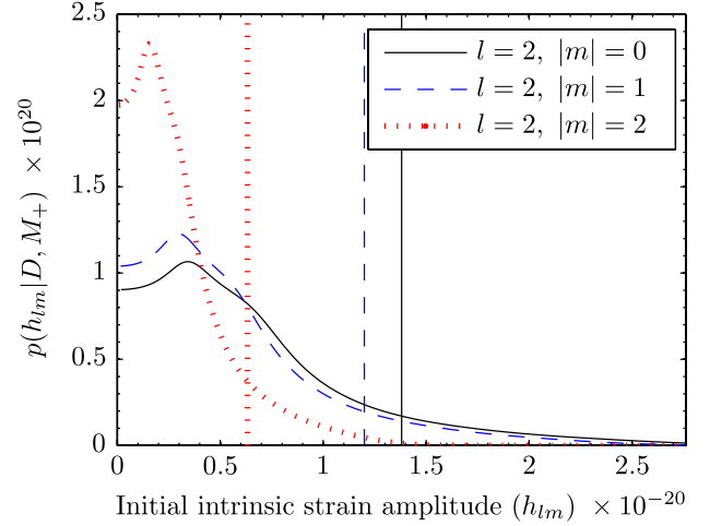
FIG. 3 (color online). The posterior probability density distributions and upper limits on the intrinsic peak amplitude of ring-downs, assuming only a single harmonic (i.e. value of |m| ) is excited. The upper limits for each harmonic are shown as the vertical lines in the figure. The numerical values of the 90% confidence upper limits can be found in Table IV. The l = 2 , |m| = 0 posterior is shown as the solid (black) line, the dashed curve (blue in the online version) shows the l = 2 , |m| = 1 posterior and the l = 2 , |m| = 2 posterior is shown as the dotted curve (red in the online version).
