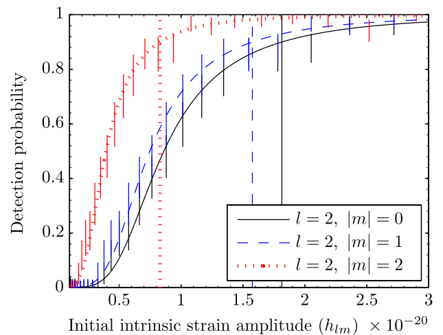
FIG. 5 (color online). Detection probabilities for software injections of ring-downs described by Eq. (10) and with parameters drawn from the prior distributions used in the search and described in Sec. IV A. Efficiencies are computed by counting the number of detections in discrete bins in amplitude. The three different curves correspond to the different harmonics (values of |m| ). The long vertical lines indicate the 90% detection efficiencies for the different harmonics, whose numerical values are given in the text. The shorter vertical bars indicate 90% binomial confidence intervals in the estimate of the detection probability in each amplitude bin. The color-coding and line-style convention is the same as that in Figs. 3 and 4: The l = 2, |m| = 0 efficiency curve is shown as the solid black line, the dashed curve (blue in the online version) shows the l = 2, |m| = 1 efficiency curve and the l = 2, |m| = 2 efficiency curve is shown as the dotted curve (red in the online version).
