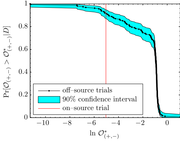
FIG. 2 (color online). The cumulative probability distribution function (CDF) for the off-source value of \ln \mathcal{O}_{(+,-)} . \ln \mathcal{O}_{(+,-)}^* indicates the observed value. The shaded region shows the 90% confidence interval on the estimate of the CDF. The vertical line (red in the online version) indicates the value of \ln \mathcal{O}_{(+,-)} = -5.03 obtained from the on-source data segment. The probability of obtaining this value or greater from background alone is 0.92, where the red line intersects the black curve. The most significant off-source trial has \ln \mathcal{O}_{(+,-)} = 1.07 , and the least significant has \ln \mathcal{O}_{(+,-)} = -11.26 .
