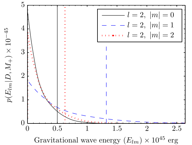
FIG. 4 (color online). The posterior probability density distributions and upper limits on the total gravitational-wave energy in the form of ring-downs, assuming only a single harmonic (i.e. value of |m| ) is excited. The upper limits for each harmonic are shown as the vertical lines in the figure. The numerical values of the 90% confidence upper limits can be found in Table IV. The l = 2 , |m| = 0 posterior is shown as the solid black line, the dashed curve (blue in the online version) shows the l = 2 , |m| = 1 posterior, and the l = 2 , |m| = 2 posterior is shown as the dotted curve (red in the online version).
