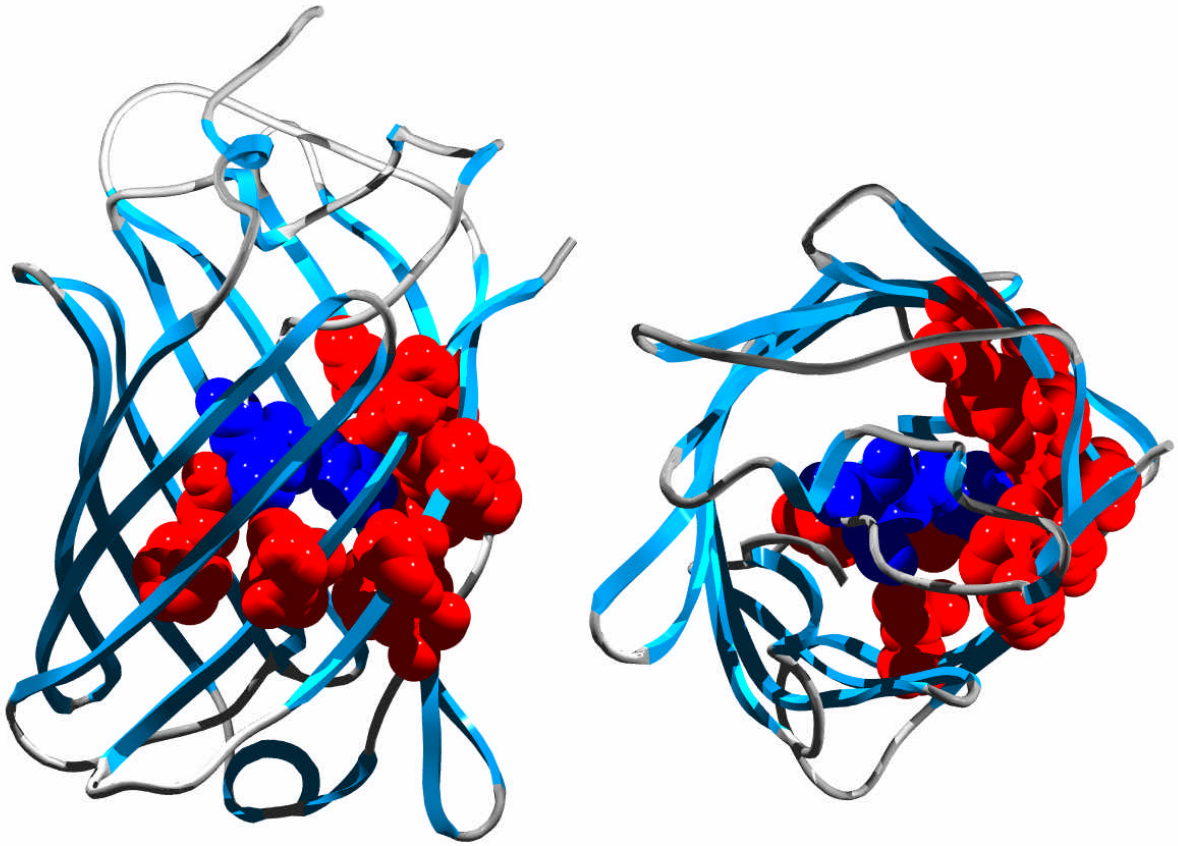
Supplementary Figure 1. Crystal structure of BFP with chromophore (blue) and targeted residues (red).
