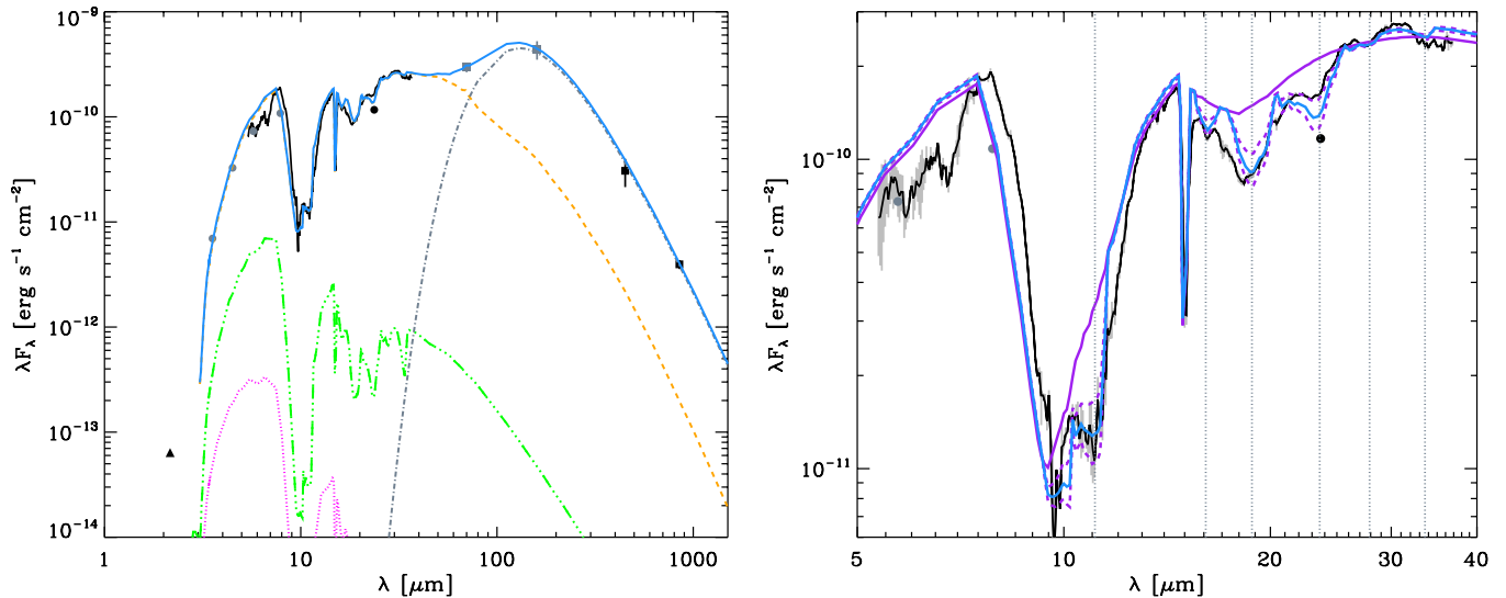
Figure 3. Left panel: best-fit model compared to the observed SED of HOPS-68. The composite SED includes the Spitzer -IRS spectrum, PANIC K_s -band flux (J. J. Tobin 2009, private communication), IRAC 3.6, 4.5, 5.8, and 8.0 \mu\text{m} and MIPS 24 \mu\text{m} fluxes (S. T. Megeath et al. 2011, in preparation), Herschel -PACS 70 and 160 \mu\text{m} fluxes ( F_\nu = 6.9 and 23.3 Jy, respectively), and SCUBA 450 and 850 \mu\text{m} fluxes (Johnstone & Bally 1999). The SCUBA estimates represent peak fluxes assuming a point-like source. The model (blue line) includes contributions from the central protostar (magenta line), the disk (green line), and the envelope (orange line); the displayed disk and central protostar components are attenuated by the envelope. In addition, a graybody (dash-dotted line) is also included to simulate external heating of the outer envelope. Right panel: close-up of the 5–40 \mu\text{m} region with IRS uncertainties (gray lines) and forsterite wavelength positions indicated (dotted lines). Envelope models with increasing crystallinity (violet lines; 0.0, 0.13, and 0.20, respectively) are shown for comparison against the best-fit model (blue line; 0.17). The mismatch near 8–9 \mu\text{m} between the adopted “astronomical” silicates and the observed amorphous silicate feature has been noted in the literature (Henning 2010). (A color version of this figure is available in the online journal.)
