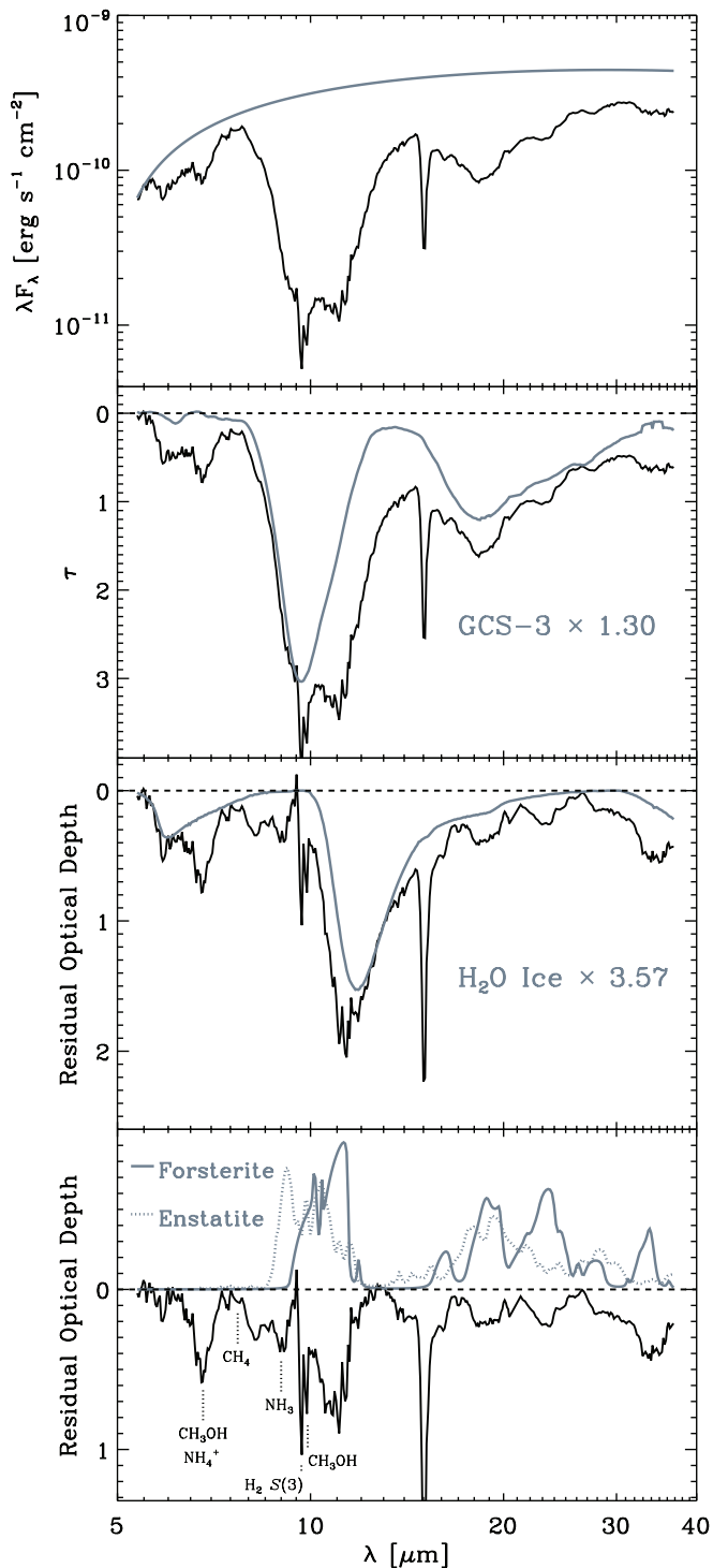
Figure 2. Isolation of crystalline silicate features in the spectrum of HOPS-68. Top panel: the Spitzer -IRS spectrum with the adopted second-order polynomial unabsorbed continuum (gray line). Second panel: the derived optical depth spectrum compared to the amorphous silicate profile of GCS-3 (gray line; Chiar & Tielens 2006). Third panel: the residual optical depth spectrum, after subtracting the scaled amorphous silicate profile of GCS-3, compared to a laboratory spectrum of pure crystalline H 2 O ice at T = 140 K (gray line; Hudgins et al. 1993). Bottom panel: the residual optical depth spectrum after subtracting the scaled H 2 O ice profile. Arbitrarily scaled mass absorption coefficients for forsterite (solid gray line) and enstatite (dotted line) are shown for comparison; these were calculated using optical constants from Sogawa et al. (2006) and Jäger et al. (1998), respectively.
