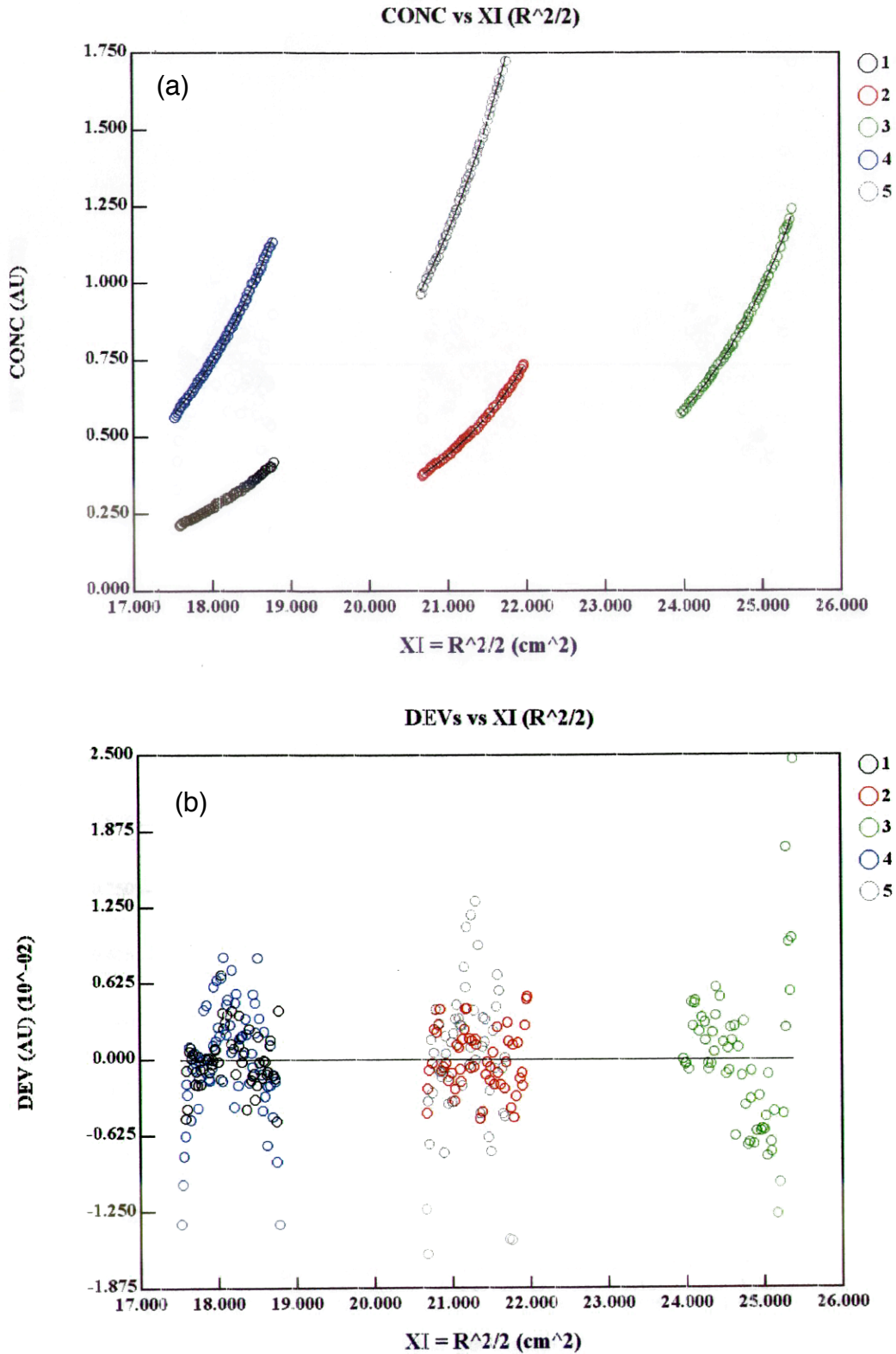
Analytical ultracentrifugation data of GB1A/GB1B complex with fits. (a) Raw data collected at 28,000 rpm with fits. Colored datapoints correspond to different concentrations. (b) residual plot of the fits.
