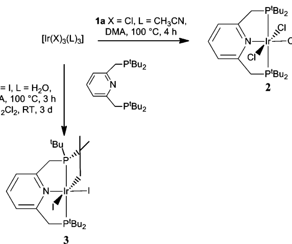
Fig. 1 Synthesis of the complexes 2 and 3 .
