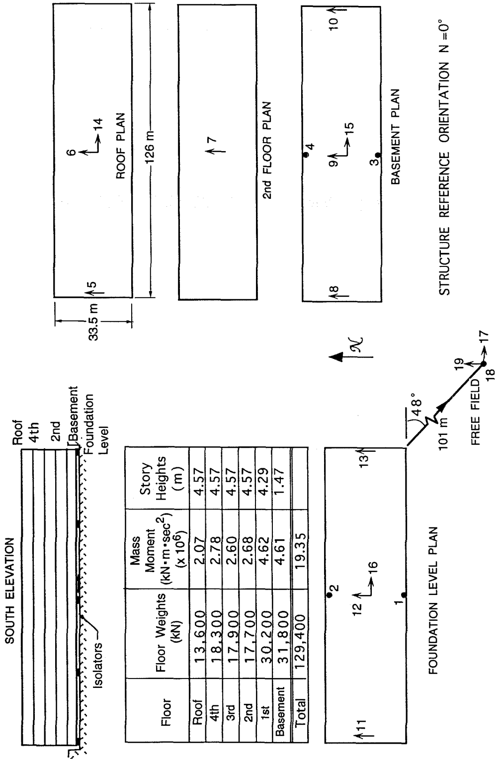
Figure 3.5 FCLJC schematic diagram showing locations of accelerometers as well as properties used in analysis.
