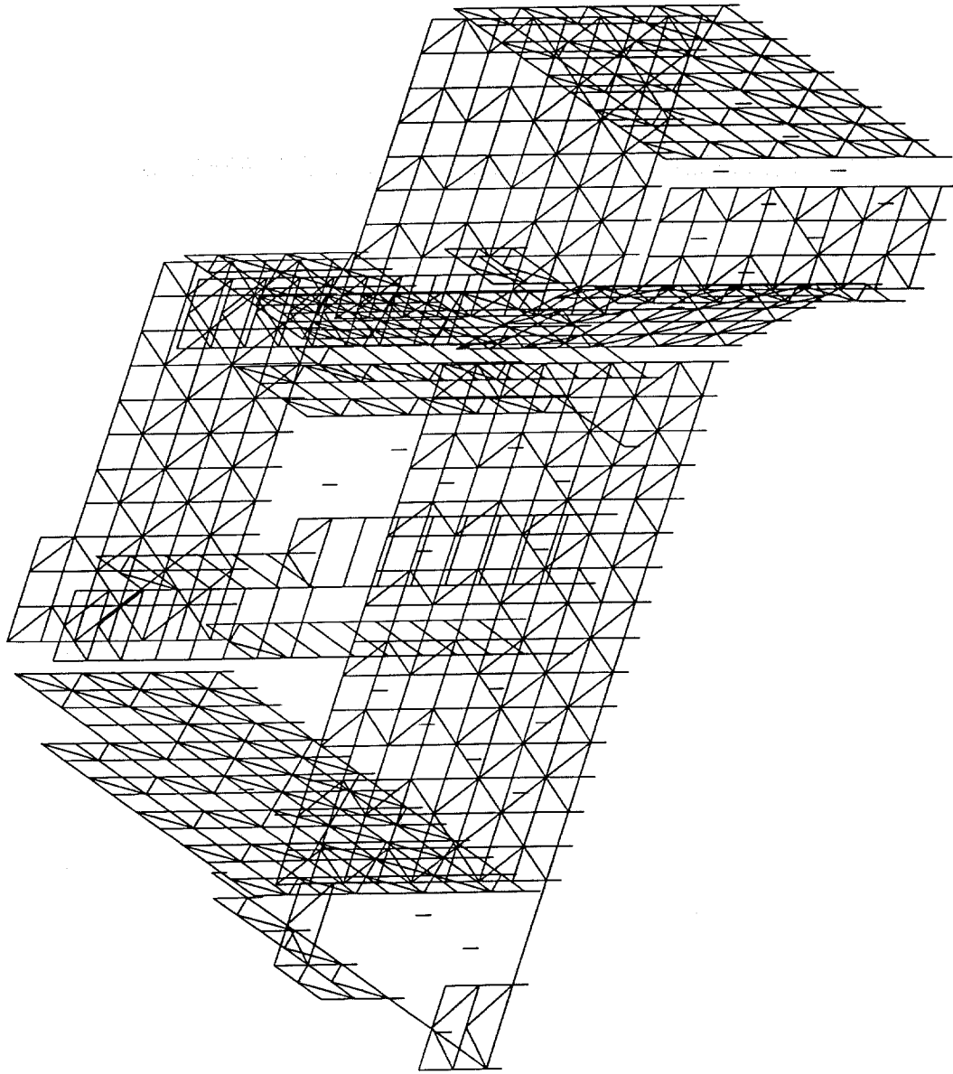
Figure 4.6 USCUH three dimensional model. Linear-elastic superstructure model supported by 149 nonlinear isolation bearings.
