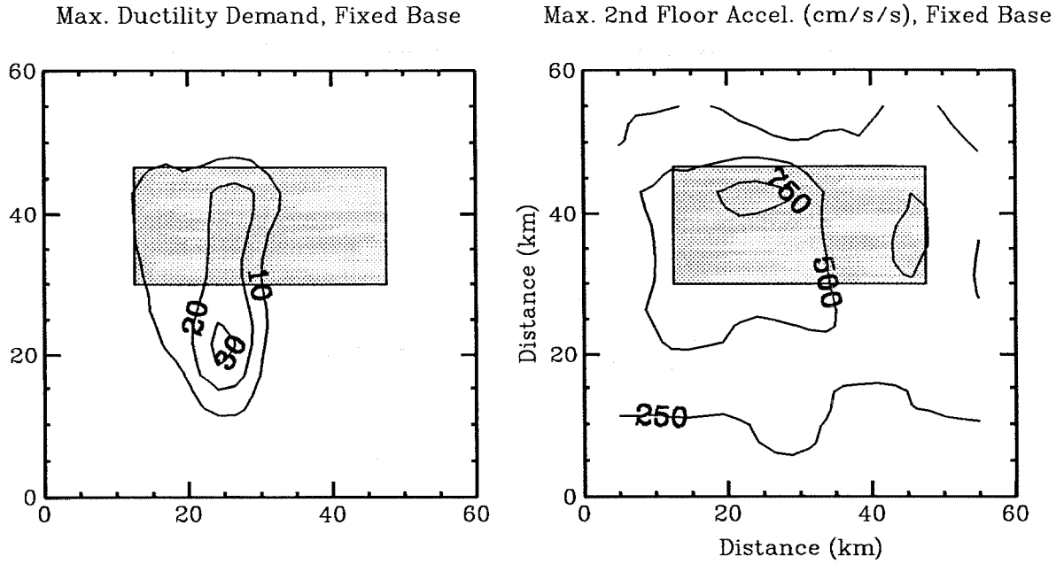
Figure 7.18 TBIB-Fixed-base contours of maximum ductility demand, and maximum second floor acceleration using the complete set of synthetic motion stations.
