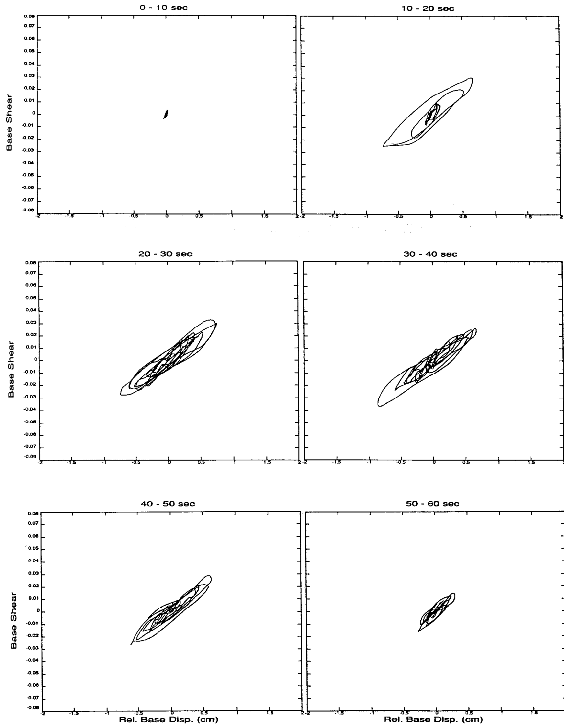
Figure 4.45 USCUI recorded force-displacement curve for the base level (isolation bearings) in the transverse direction from the 1992 Landers earthquake which has been divided into 10 sec time segments (Refer to equation 4.7).
