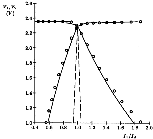
Figure 5 Experimental data (circles) and theoretical statements (solid lines) for a two-neuron winner-take-all circuit with a channel length for transistors T_{1_1} and T_{1_2} of 3\mu\text{m} . The dotted lines show the losing response for the circuit used in Figure 3, which has a channel length for transistors T_{1_1} and T_{1_2} of 13.5\mu\text{m} .
