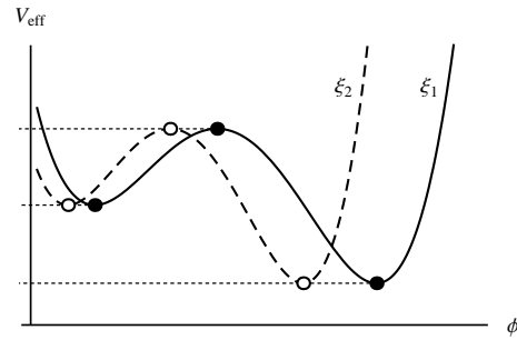
FIG. 2: A schematic illustration of the behavior of the exact effective potential as the gauge parameter \xi is varied according to Nielsen's identity. The values of the potential at its extrema stay unchanged but the fields extremizing the potential are gauge-dependent.
