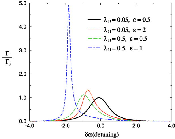
FIG. 2. The ratio of \Gamma/\Gamma_0 as a function of detuning at different values of driving strength and self-anharmonicity (Kerr effect coupling). The parameters are presented in units of the damping rate \kappa .
