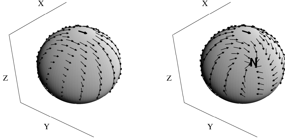
Figure 2: Transport maps on S^2 . We depict the vector \mathcal{T}_{(q,r)}\dot{r} for two different transport maps: on the left our smooth global design, on the right a design based on a latitude, longitude chart, with the north pole denoted by the letter N.
