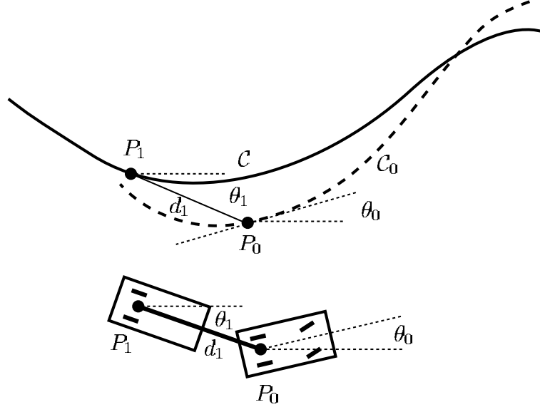
Figure 10: case n = 1 .
