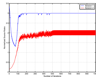
Fig. 7. The evolution of source rates with step size \gamma_t = 0.01 for the example network without given coding subgraph.
