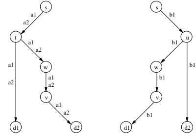
Fig. 3. Multicast trees for the example shown in Fig.1. Coding is done on the shared link (w, v) , which, as part of the left tree, has one downstream destination d_2 , and, as part of the right tree, has one downstream destination d_1 . The left tree can support up to two units of information flow and the right tree can independently support up to one unit of information flow, since coding on link (w, v) allows the two trees to share capacity.
