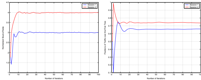
Fig. 5. The evolution of source rates versus the number of iterations of tree adaptation algorithm(left panel) and the evolution of traffic split vectors (right panel) with stepsize \kappa_{\gamma_t} = 0.01 for the example network with given coding subgraphs.
