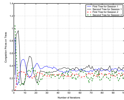
Fig. 6. The evolution of congestion prices over different multicast trees versus the number of iterations of the tree adaptation algorithm.
