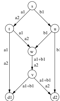
Fig. 1. An example network coding subgraph with one source s and two destinations d_1 and d_2 . Links (s, u) , (u, w) and (u, d_2) are assumed to have one unit of capacity, and all other links have two units of capacity.
