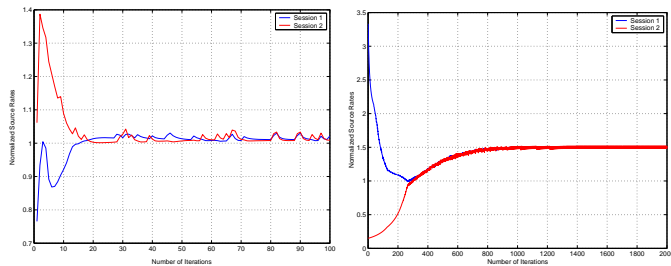
Fig. 8. The evolution of source rates for the case with given coding subgraph (left panel) and for the case without given coding subgraph (right panel).
