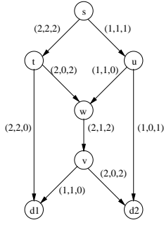
Fig. 2. Flow variables for network code shown in Fig.1. Each link (i, j) is marked by the triple (f_{i,j}, g_{i,j}^{d_1}, g_{i,j}^{d_2}) .
