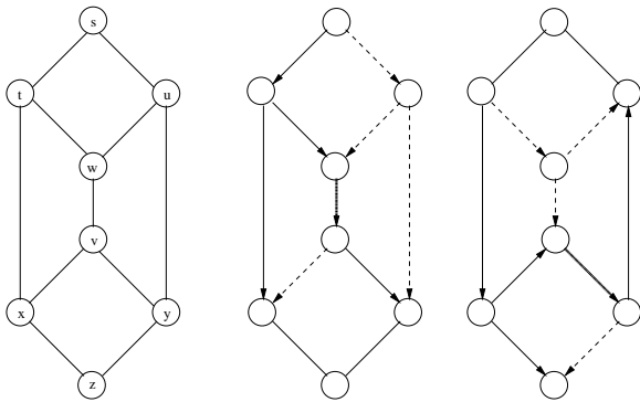
Fig. 4. A simple network with two multicast sessions. The given coding subgraphs for sessions 1 and 2 are shown in the middle and right graphs respectively. For each session, the first tree is indicated by solid arrows, the second by dashed arrows, and the overlapping segments by bold arrows.
