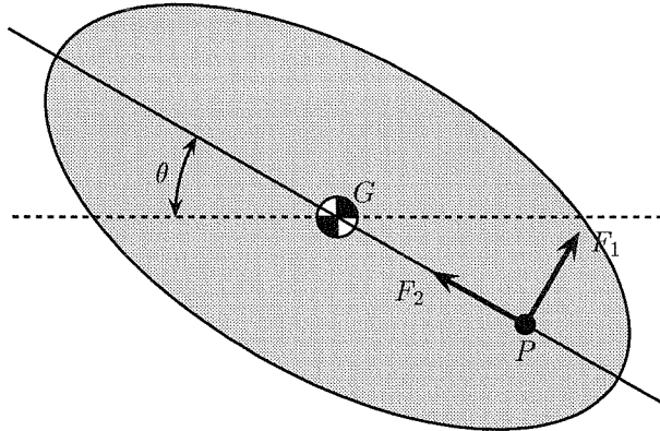
Figure 2: Underwater vehicle in \mathbb{R}^2
