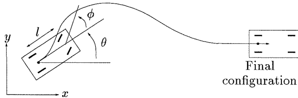
Figure 1: Path Planning for Kinematic Car
