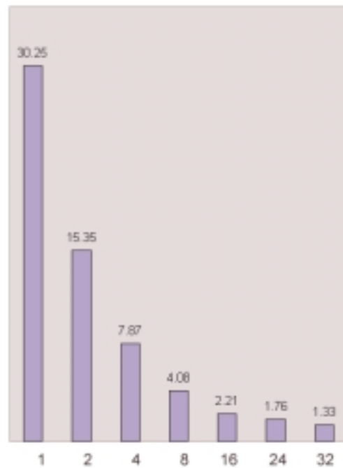
Figure 3: Wall clock time in seconds per one time-step vs. the number of system processors.
