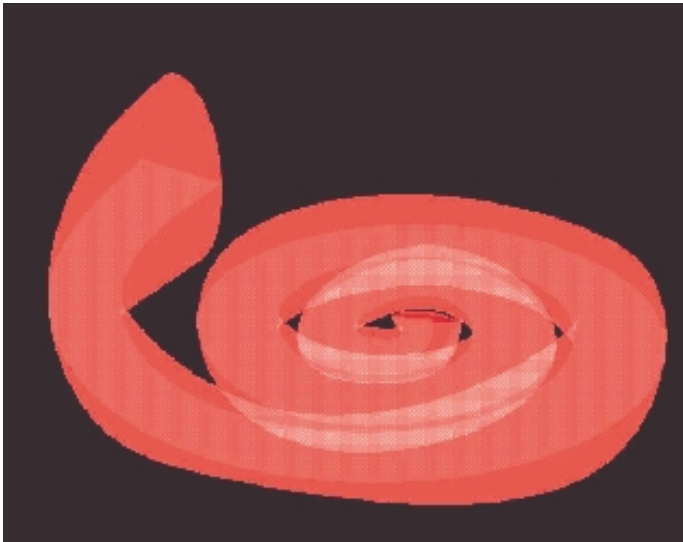
Figure 1 Partially transparent cochlea model as seen from the outside.
