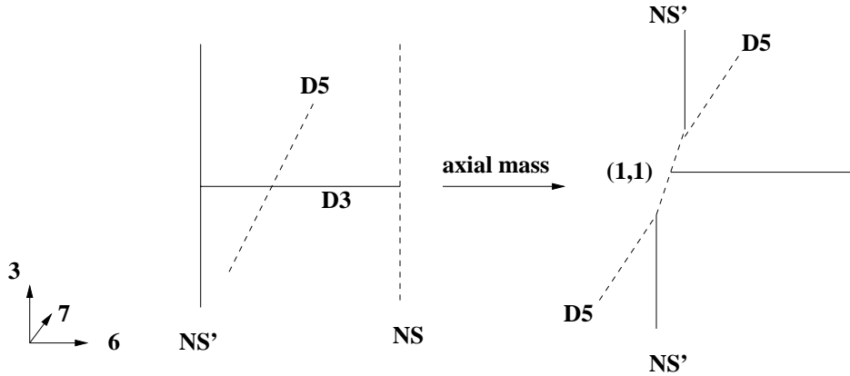
Figure 1: Turning on an axial mass for the electron.
