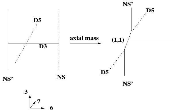
Fig.1. Turning on an axial mass for the electron.
