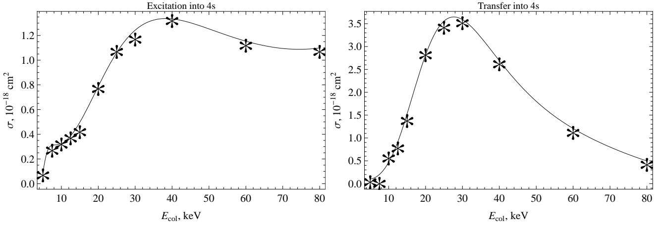
Figure B4. Cross sections for excitation (left panel) and charge transfer (right panel) into 4s state. Stars show results of our calculations. Solid line corresponds to our Chebyshev polynomial fit.
