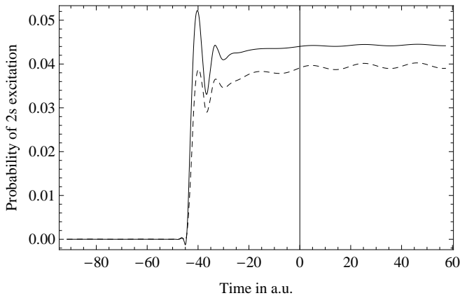
Figure 6. Probability of excitations into 2s states as a function of time for 2 different values of impact parameter b = 0.2 a.u. (solid curve) and b = 0.8 a.u. (dashed curve).
