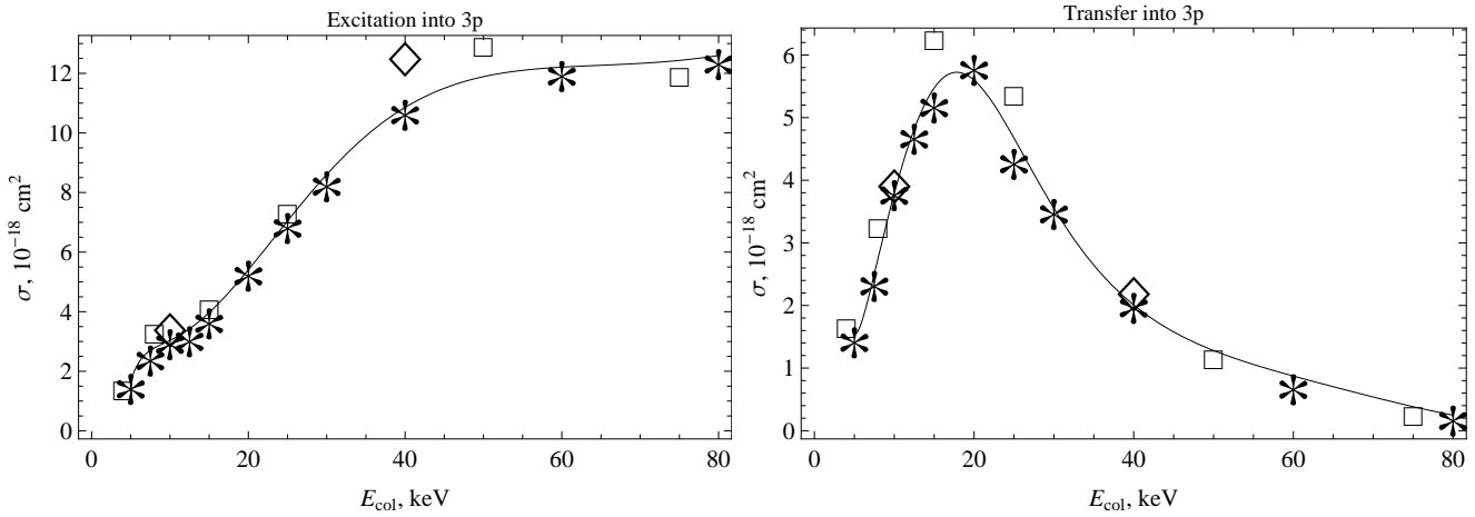
Figure B2. Cross sections for excitation (left panel) and charge transfer (right panel) into 3p state. Stars show results of our calculations, diamonds correspond to Kolakowska (1998), and squares show results from Winter (2009). Solid line corresponds to our Chebyshev polynomial fit.
