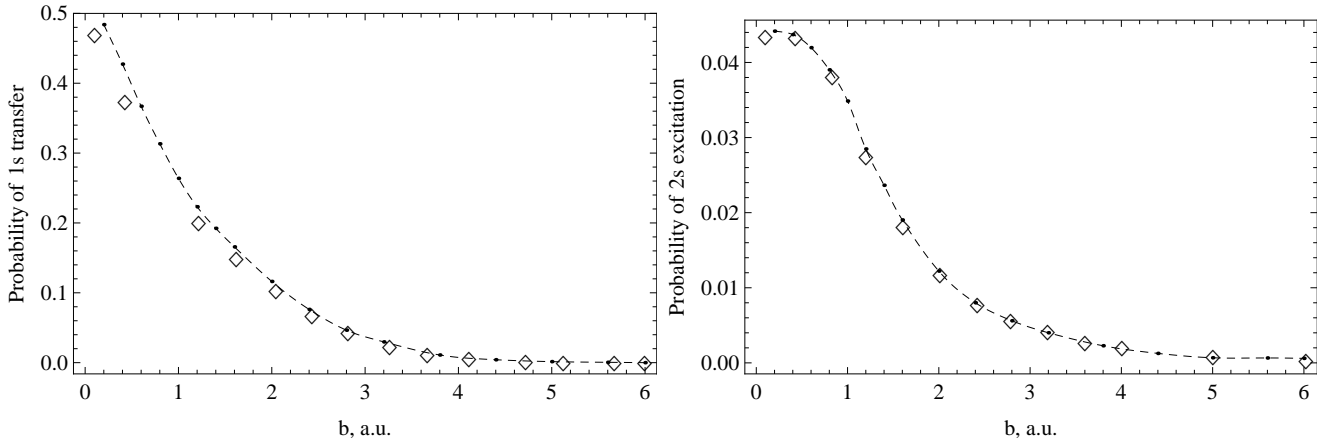
Figure 5. Plot on the left shows probability of charge transfer into 1s state as a function of impact parameter for E_{col} = 40 keV, and the plot on the right shows probability of excitation into 2s state. Diamonds show corresponding results from Kolakowska et al. (1998).
