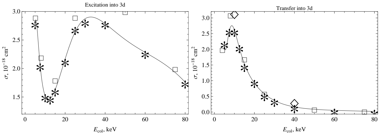
Figure B3. Cross sections for excitation (left panel) and charge transfer (right panel) into 3d state. Stars show results of our calculations, diamonds correspond to Kolakowska (1998), squares show results from Winter (2009). Solid line corresponds to our Chebyshev polynomial fit.
