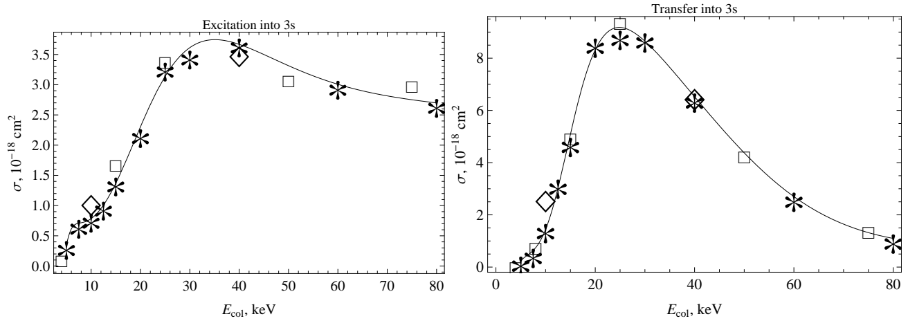
Figure B1. Cross sections for excitation (left panel) and charge transfer (right panel) into 3s state. Stars show results of our calculations, diamonds correspond to Kolakowska (1998), and squares show results from Winter (2009). Solid line corresponds to our Chebyshev polynomial fit.
