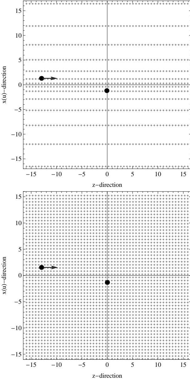
Figure 1. An example of a grid in xz -plane used in our analysis (upper panel) with every third point plotted in both x - and z -direction, so that the aspect ratio is illustrated correctly. We also show positions of the moving hydrogen atom (thick dot with the vector) and stationary proton at z = 0 . Distances between grid points in x -direction correspond to equidistant intervals ( \Delta_u = 0.2 in u -space), so that in the region close to the interacting particles \Delta_x \approx \Delta_u = 0.2 , while at large separations spacing in x -direction is significantly increased reaching, for example, \Delta_x \sim 1.6 at x \sim 16 . The lower panel shows a “brute force” Cartesian grid with \Delta_x = \Delta_z = 0.2 (again only every third point is plotted) and allows to clearly see the advantage of our grid choice.
