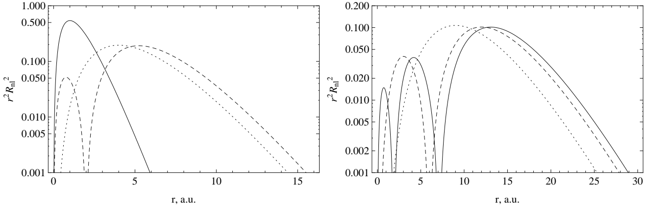
Figure 2. Plot on the left shows charge density distribution r^2 R_{nl}^2(r) for 1s (solid), 2s (dashed), and 2p (dotted) states. Plot on the right shows charge distribution for 3s (solid), 3p (dashed) and 3d (dotted) states.
