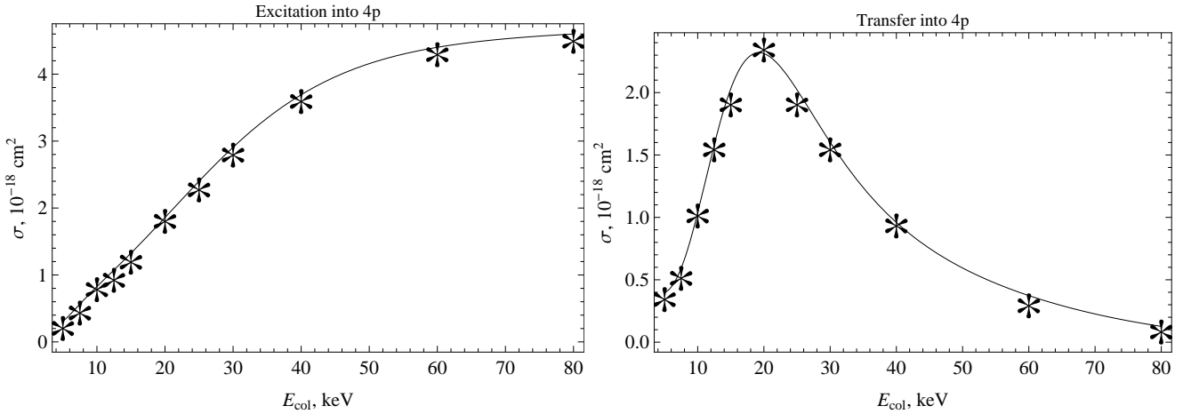
Figure B5. Cross sections for excitation (left panel) and charge transfer (right panel) into 4p state. Stars show results of our calculations. Solid line corresponds to our Chebyshev polynomial fit.
