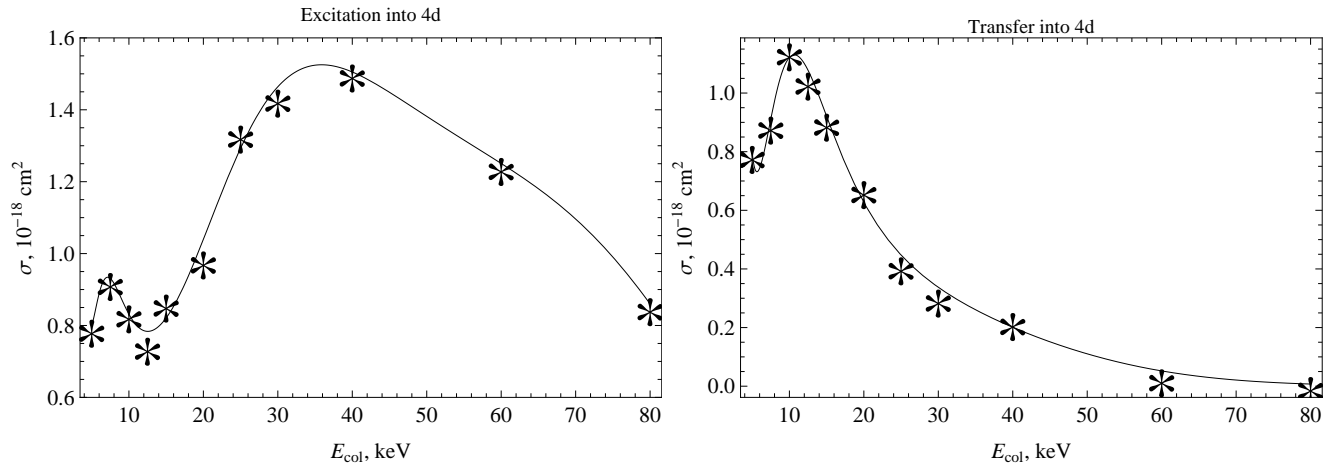
Figure B6. Cross sections for excitation (left panel) and charge transfer (right panel) into 4d state. Stars show results of our calculations. Solid line corresponds to our Chebyshev polynomial fit.
