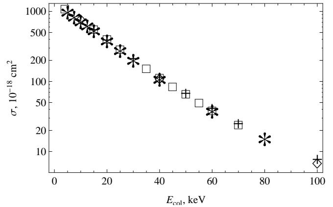
Figure 7. Excitation cross sections (in units of 10^{-18} cm 2 ) for charge transfer into 1s state. Stars show results of our calculations, diamonds correspond to Kolakowska (1998), squares show results from Winter (2009) and plus signs correspond to the results from Kuang & Lin (1996).
