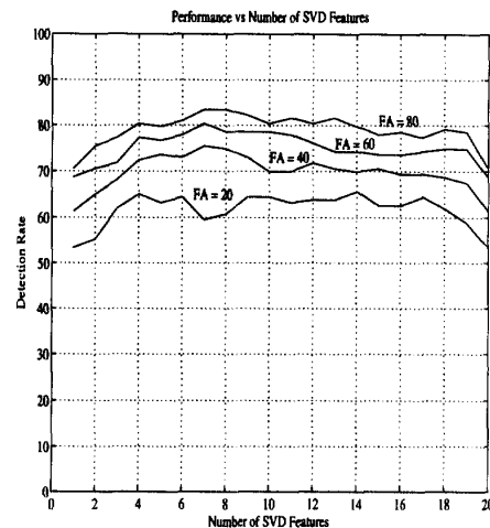
Figure 8: Empirical performance vs number of SVD features.
