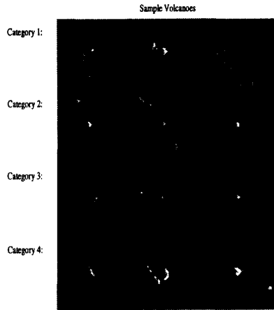
Figure 2: Volcano confidence categories.
