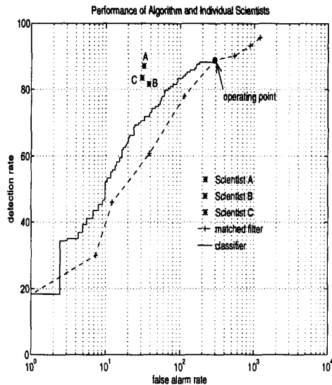
Figure 7: Performance of our algorithm compared to individual scientists.
