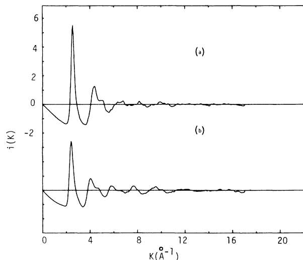
FIG. 3. The reduced interference functions i(K) = K[I(K) - 1] for (a) as-quenched Zr 3 Rh and (b) Zr 3 RhH 5.5 prepared in 1 atm H 2 at 180°C.
