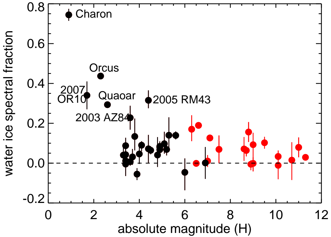
Fig. 2.— Water ice absorption as a function of absolute magnitude. Objects with semimajor axis outside of 30 AU are shown in black, while those inside of 30 AU are shown in red. Absolute magnitudes are taken from the Minor Planet Center and have typical random errors below 0.3 magnitudes
