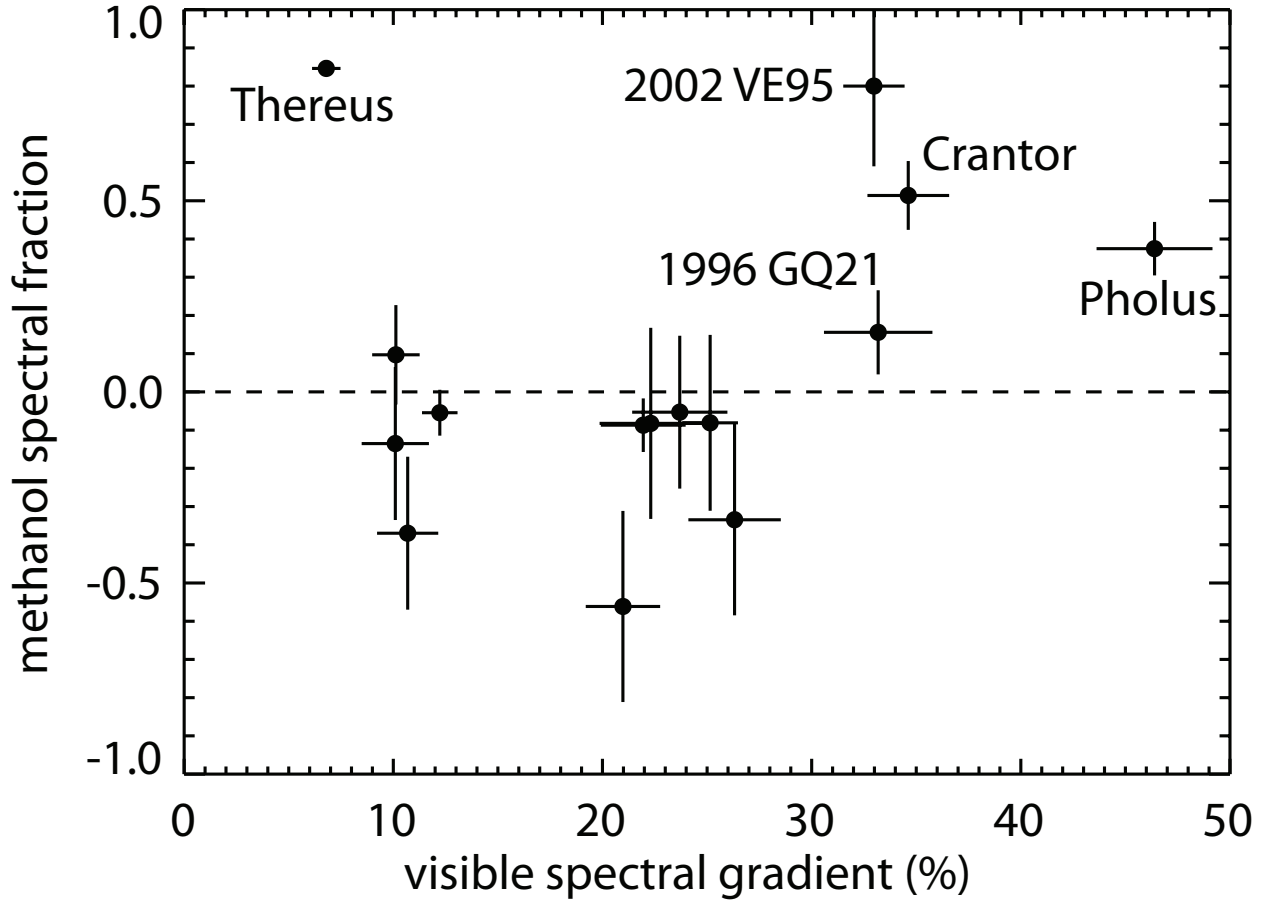
Fig. 4.— Methanol ice absorption fraction as a function of spectral color gradient. The red family shows a positive correlation between color and methanol absorption and color at the 99.8% confidence level, as would be predicted by the methanol evaporation model for KBO coloration. In the blue family, methanol is only detected on the centaur Thereus, but higher quality spectra suggest that this detection is spurious.
