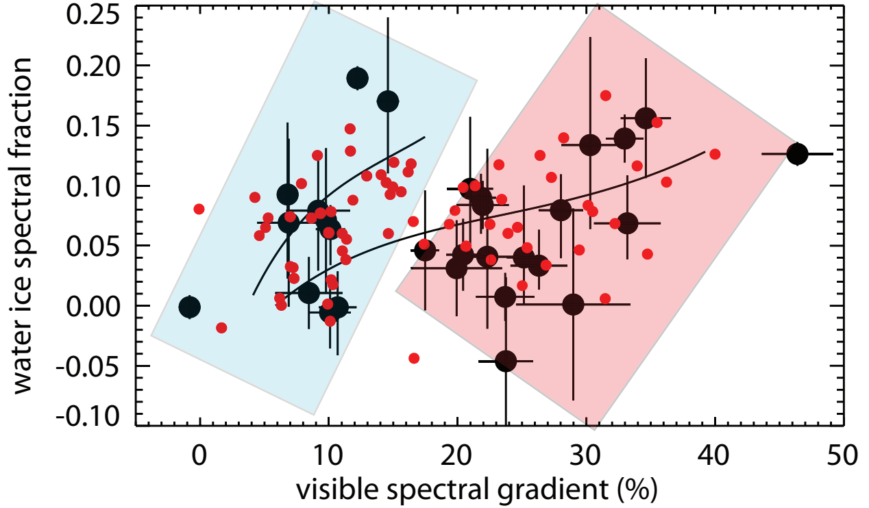
Fig. 3.— Water ice absorption fraction as a function of spectral color gradient. Black points with error bars show the spectral data and colors derived from visible photometry. The red points without error bars (typical uncertainties are smaller than those of the spectral data) are from the H/WTSOSS photometric survey of Fraser & Brown (2012) and have been transformed to these variables. The two lines show the mixing models which best fit the three-color H/WTSOSS data. The blue and red shading show the neutral and the red families of objects.
