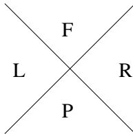
Fig. 5: Rindler coordinate patches.
