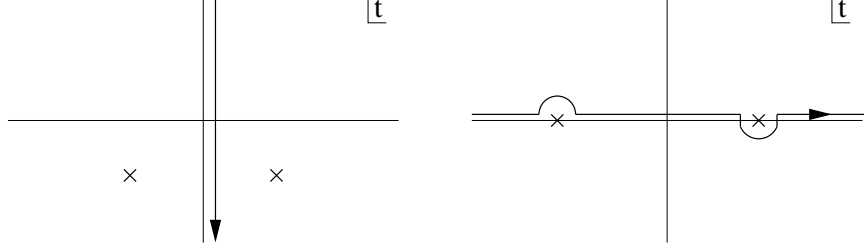
Fig. 4: Standard contour rotation defining amplitudes in Minkowski space.
