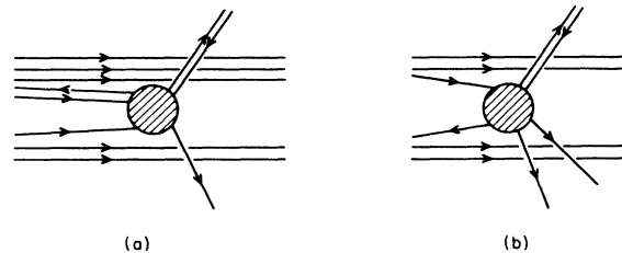
FIG. 20. Possible minimal large- p_\perp scatterings if gluon exchange is not allowed: (a) q\bar{q} \rightarrow \pi q and (b) qq \rightarrow \pi qq .
