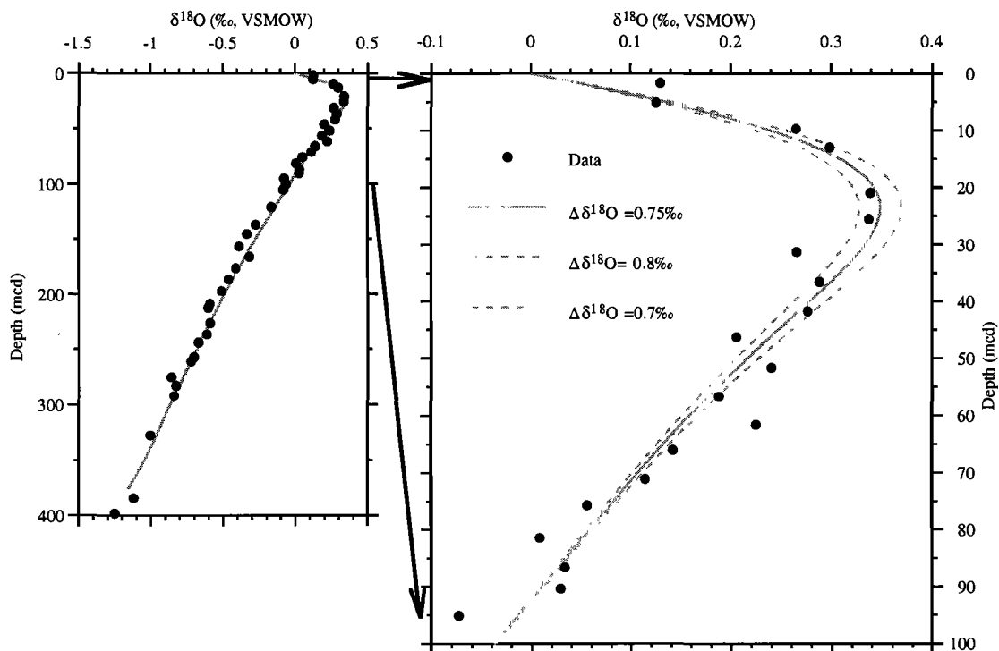
Figure 2. Plot of \delta^{18}\text{O} vs. meters composite depth in ODP core 1063A. Error bars ( 1\sigma ) are from replicate analyses of the same sample. The gray line is the best-fit model run using a glacial/interglacial change of 0.75\text{‰} . Dashed gray lines are the results of changing the 0.75\text{‰} fit by \pm 0.05\text{‰} .
