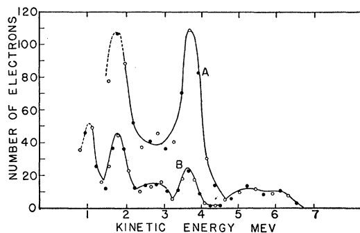
FIG. 2. Curve A , the distribution in kinetic energy of 450 electrons ejected from a carbon lamina 0.12 cm thick within an angle of 20^\circ with the forward direction of the radiation, measured in fields of 1500 and 1000 gauss, and plotted in overlapping intervals of 0.46 Mev. Curve B contains that portion of the electrons measured in the 1000 gauss field. The curves have been broken in the regions of low resolving power.
