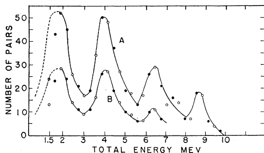
FIG. 1. Curve A , the distribution in total energy of 300 positron-electron pairs ejected from 0.033 cm lead foil by the radiation from B+D measured in fields of 1700 and 1000 gauss, and plotted in overlapping intervals of 0.57 Mev. Curve B contains that portion of the pairs measured in the 1000 gauss field. The dotted portions indicate by how much the low energy component has been broadened to account for those low energy pairs which have been lost in the measuring process.
