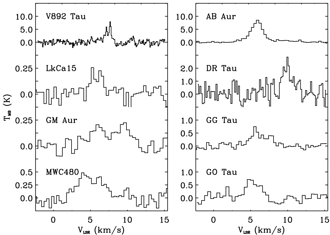
FIG. 9.—As Fig. 6, but for CO 6–5 CSO spectra
