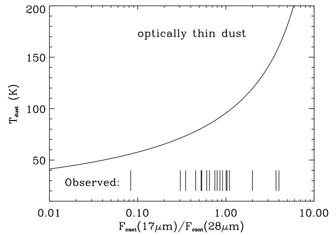
FIG. 4.—Dust temperature as a function of the ratio of the continuum fluxes at 17 and 28, assuming optically thin emission. The vertical bars at the bottom indicate the observed ratios for our sources. The errors on the ratio are typically 50%.
