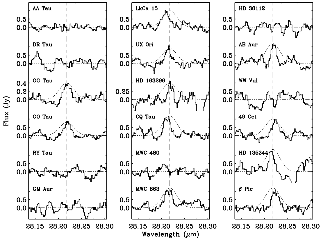
FIG. 1.—H 2 S(0) 28 \mu m spectra observed with the ISO-SWS toward pre-main-sequence and debris-disk stars. The underlying continuum has been subtracted. The rest wavelength of the J = 2-0 transition is indicated by the dashed line. Small wavelength shifts may be attributed to instrumental effects (see text). The dash-dotted Gaussian corresponds to emission by a source filling the beam; the H 2 lines have to lie inside this Gaussian to be considered detected.
