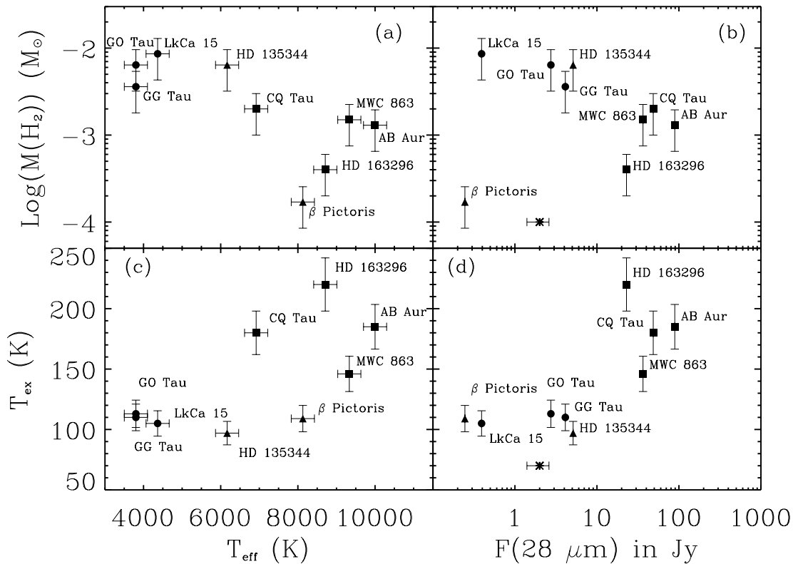
FIG. 14.—Panels (a) and (c) show the warm gas mass derived from H 2 and the corresponding H 2 excitation temperature as a function of the effective temperature of the central star. Panels (b) and (d) plot the variation of the warm gas mass and excitation temperature against the continuum flux at 28 \mu\text{m} normalized at 100 pc.
