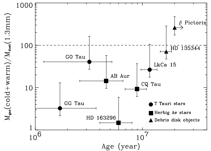
FIG. 13.—Evolution of the ratio of the total gas mass to the solid mass in circumstellar disks. The standard interstellar ratio is 100:1.
