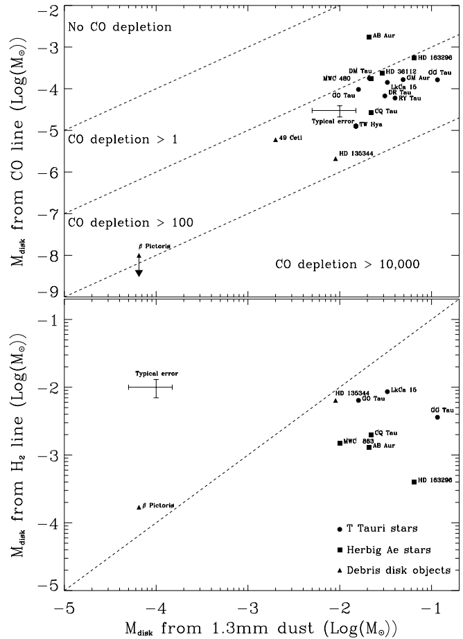
FIG. 10.—Estimated gas mass obtained from CO observations (upper panel) and \text{H}_2 observations (lower panel) plotted against the disk mass computed from 1.3 mm dust assuming a gas/dust ratio of 100:1. In the upper panel, the dashed lines separate the regions of different CO depletion factors.
