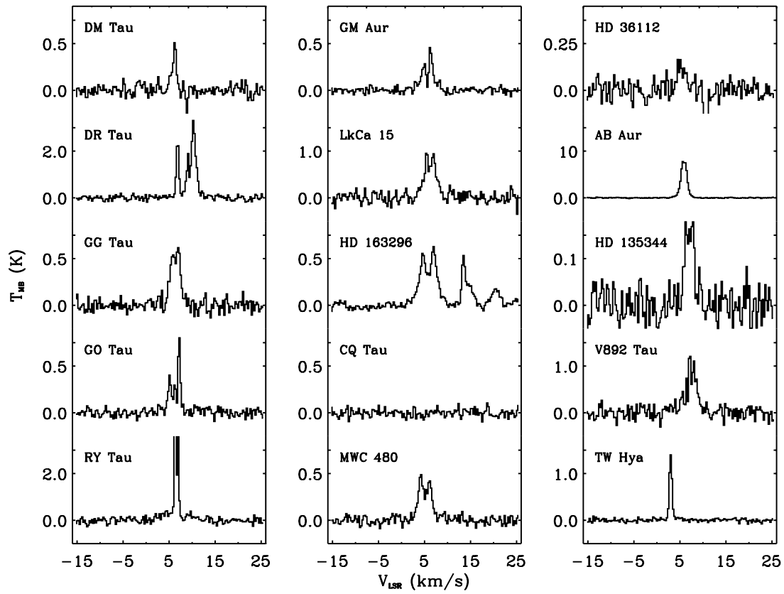
FIG. 6.—Single-dish JCMT spectra of the ^{12}\text{CO} 3–2 line at 345 GHz toward protoplanetary disks. The vertical scale is T_{\text{MB}} in K. The horizontal scale denotes the LSR velocity. The characteristic double-peaked line profile due to a rotating disk is seen for many sources.
