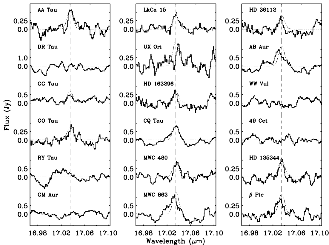
FIG. 2.—As Fig. 1, but for the H_2 S(1) J = 3-1 transition
