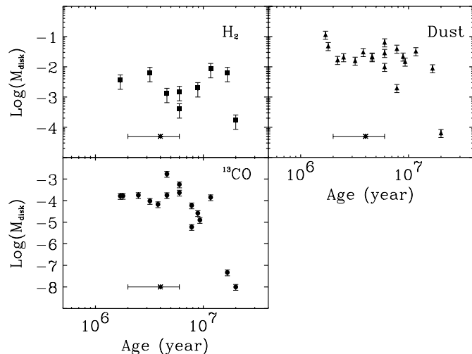
FIG. 12.—Variation of the total disk mass with the age of the central object deduced from the three methods.
