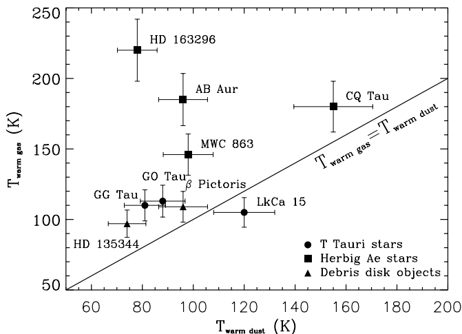
FIG. 5.—Warm gas temperatures vs. warm dust temperature for sources having both S(0) and S(1) lines detected. The errors on the temperatures are \sim 10\% .
