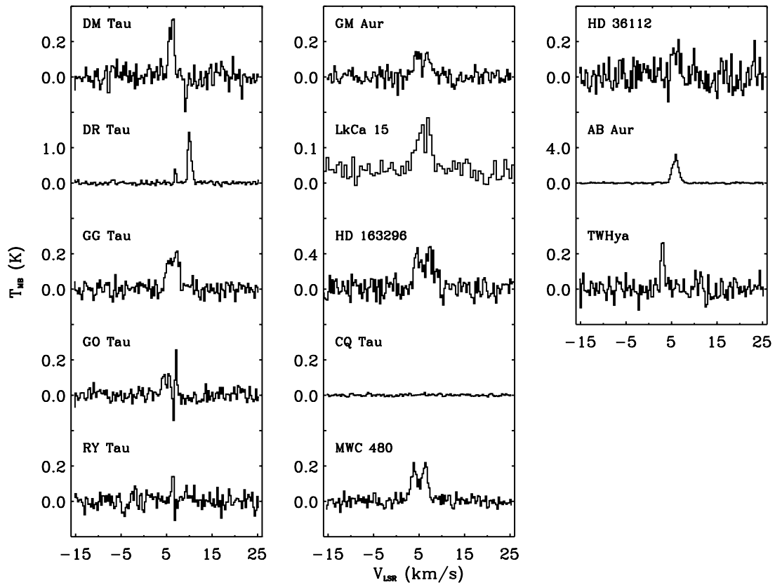
FIG. 7.—As Fig. 6, but for ^{13}\text{CO} 3–2 JCMT spectra
