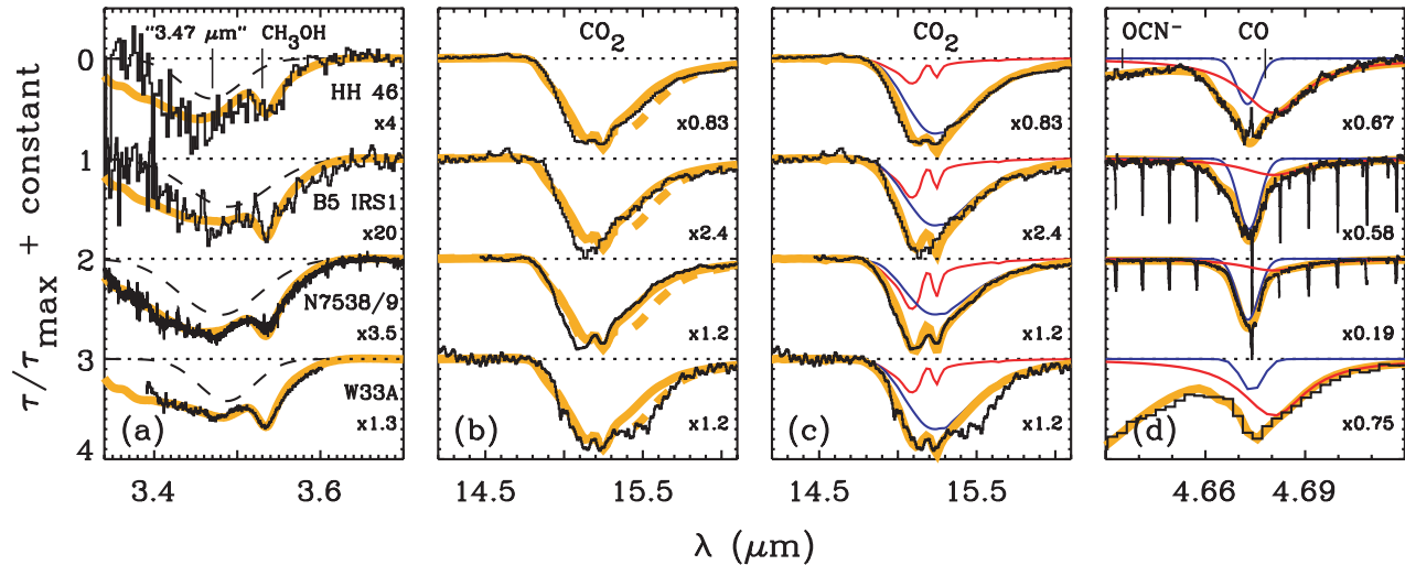
FIG. 2.—Solid \text{CH}_3\text{OH} , \text{CO}_2 , and \text{CO} spectra of HH 46 IRS and B5 IRS 1 compared with the massive protostars NGC 7538 IRS 9 and W33A in each panel (top to bottom). The normalization factor is indicated in the right corner of each plot. (a) A laboratory pure \text{CH}_3\text{OH} spectrum at T_{\text{lab}} = 10 K (thick yellow line) to which is added a Gaussian (dashed line) to account for the underlying “3.47 \mu\text{m} ” absorption feature. The NGC 7538 IRS 9 and W33A data are from Boogert et al. (2004) and Brooke et al. (1999), respectively. (b) The \text{CO}_2 bending mode observed with Spitzer IRS (HH 46 IRS and B5 IRS 1) and ISO SWS (NGC 7538 IRS 9 and W33A). The thick yellow dashed line is the laboratory ice \text{H}_2\text{O}:\text{CH}_3\text{OH}:\text{CO}_2 = 0.84:0.92:1 , and the solid thick, yellow line is a laboratory ice with reduced \text{CH}_3\text{OH} content, \text{H}_2\text{O}:\text{CH}_3\text{OH}:\text{CO}_2 = 0.92:0.29:1 , both at T_{\text{lab}} = 115 K. Only for W33A is an enhanced \text{CH}_3\text{OH}:\text{CO}_2 ratio required, in agreement with the strong 3.53 \mu\text{m} \text{CH}_3\text{OH} feature in (a). (c) The \text{CO}_2 bending mode for the same sources as in (b), but now fitted with different laboratory spectra: a highly processed polar ice ( T_{\text{lab}} = 125 K; red line) in combination with an \text{H}_2\text{O} -rich, \text{CH}_3\text{OH} -deficient cold ice ( T_{\text{lab}} = 10 K; blue line). The sum of these two components is the thick yellow line. (d) The absorption band of solid \text{CO} observed with VLT ISAAC (HH 46 IRS), Keck NIRSPEC (B5 IRS 1 and NGC 7538 IRS 9), and ISO SWS (W33A). Narrow absorption lines are due to circumstellar gas-phase \text{CO} . The onset of the 4.62 \mu\text{m} “XCN” band is seen in HH 46 IRS and W33A. Gaussian and Lorentzian fits to the apolar and polar \text{CO} components are indicated by blue and red lines (Pontoppidan et al. 2003b). The thick yellow line represents the combined fit, including the XCN band and a blueshifted \text{CO} component, which are not shown separately.
