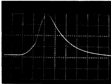
FIG. 1. Light output of a \text{Ca}(\text{NbO}_3)_2:\text{Nd}^{3+} crystal at 1.060 \mu , just above threshold observed with a PbS cell. The time scale is 100 \mu\text{sec}/\text{div} .
