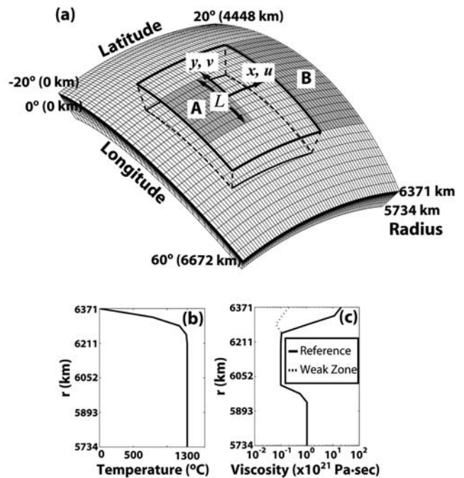
Figure 2. (a) Coordinates of the finite element mesh and configuration for boundary conditions. The inner region is the volume outlined by thick solid and dashed lines. x -axis is along the 30^\circ meridian and y -axis along the equator. u and v are velocity tangential to x - and y -axis, respectively. Velocity boundary conditions are applied on the regions shaded with dark gray: u = 0.0 , v = v_0 = 5.0 cm/yr in region A, while u = v = 0 in region B. v = 0.0 and \partial u/\partial x = 0.0 on the vertical boundaries. The mesh has 32 elements in longitude and 64 in latitude (with regular spacing) and 16 in depth (refined through the upper 100 km) (b) Variations of temperature with depth. (c) Viscosity variation with depth. Viscosity for the blocks is drawn in solid line. Viscosity for a weak zone with viscosity ratio \eta_{\text{weak}}/\eta_{\text{normal}} of 10^{-2} is drawn in dashed line.
