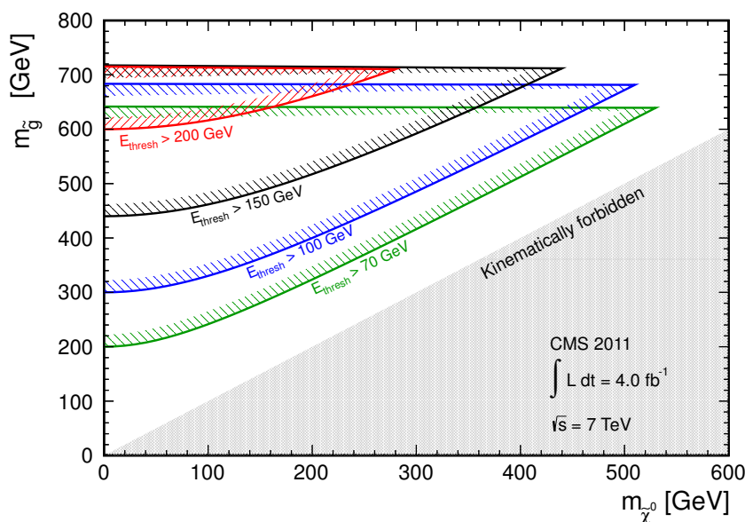
Figure 5. The region of m_{\tilde{g}} - m_{\tilde{\chi}_1^0} excluded by the analysis, valid for gluino lifetimes 10^{-5} \text{s} < \tau_{\tilde{g}} < 10^3 \text{s} , using several jet energy thresholds E_{\text{thresh}} .
