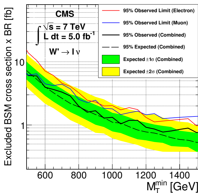
Figure 4. 95% confidence level upper limits on the cross section times branching fraction for physics beyond the SM (labelled BSM) for the charged lepton-neutrino production with transverse masses exceeding M_T^{\min} . The results for the electron, the muon channel, as well as for both channels combined are presented. The one (two) sigma uncertainty bands are shown in green (yellow).
