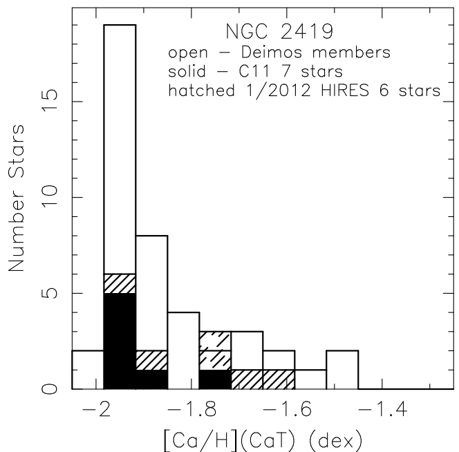
Figure 2. A histogram of [\text{Ca}/\text{H}] as inferred from the near-IR Ca II triplet line strengths in the DEIMOS moderate resolution spectra of C10 is shown for the sample of 43 definite members of NGC 2419 isolated in that paper. The sample from C11 of 7 RGB stars in this GC with HIRES spectra is shown by the solid fill. The 6 additional NGC 2419 stars presented here are indicated by the hatched areas.
