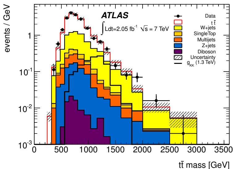
Figure 6. Reconstructed invariant mass distribution of the t\bar{t} candidates after signal selection. The e +jets and \mu +jets channels are combined. The shaded band indicates the uncertainty in the normalization of the Standard Model prediction, but does not include the shape uncertainty or the impact of uncertainties on reconstructed objects. The variable bin size is chosen to match the mass resolution for a resonant signal.
