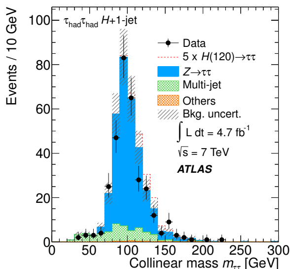
Figure 7. Reconstructed m_{\tau\tau} of the selected events in the H \rightarrow \tau_{\text{had}}\tau_{\text{had}} channel. Expectations from the Higgs boson signal ( m_H = 120 \text{ GeV} ) and from backgrounds are given. Results are shown after all selection criteria (see text). For illustration only, the signal contribution has been scaled by a factor given in the legend.
