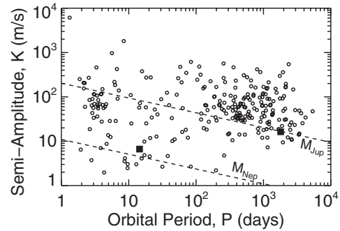
Figure 8. Velocity semi-amplitude vs. orbital period for planets with radial velocity detections. The two planets announced in this paper are indicated by filled squares. Diagonal dashed lines show the approximate locus of Jupiter- and Neptune-mass planets, assuming M = M_{\odot} , e = 1 , and \sin i = 1 . Detecting low-mass planets with long periods is particularly challenging.
