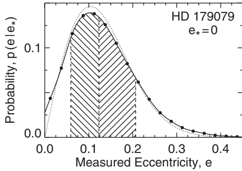
Figure 6. Probability that we would measure an eccentricity e for our 74 Keck observations of HD 179079, if the true eccentricity is zero, e_* = 0 . The asymmetric distribution of measured eccentricities has a median of 0.123 and a standard deviation of 0.075, despite a true eccentricity of zero. The hatched regions show 34.1% of the distribution on either side of the median.
