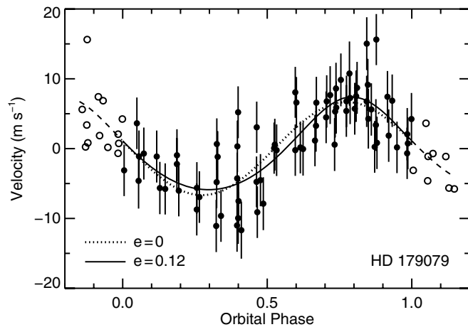
Figure 3. Phased radial velocities for HD 179079 reveal an orbital period of 14.48 days, a velocity amplitude of 6.64 \text{ m s}^{-1} , and an eccentricity of 0.12. Error bars illustrate the quadrature sum of the velocity precision for each measurement and 3.5 \text{ m s}^{-1} of jitter (systematic errors and/or intrinsic stellar variability). The Keplerian model is overplotted with a solid line and the dotted line shows the model with eccentricity fixed to zero. Adopting a stellar mass of 1.15 M_{\odot} we derive a planet mass, M \sin i = 28 M_{\oplus} , and orbital radius of 0.122 AU.
