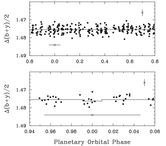
Figure 4. Top panel: the 243 ensemble D - (A + B + C)/3 photometric observations of HD 179079 in the combined Strömgren (b + y)/2 passband, acquired with the T12 0.8 m APT over two observing seasons and plotted modulo the 14.476 d orbital period of the inner companion. Phase 0.0 corresponds to a predicted time of mid-transit. A least-squares sine fit at the orbital period yields a semiamplitude of only 0.00007 \pm 0.00016 mag. Bottom panel: the photometric observations of HD 179079 near the predicted time of transit plotted with an expanded scale on the abscissa. The solid curve shows the predicted time of transit with a drop in stellar brightness of 0.08% ( \sim 0.00087 mag). The error bar in the upper right of both panels represents the mean precision of a single observation (0.0019 mag). The error bar immediately below the predicted time of transit in both panels represents the uncertainty in the predicted time of mid-transit ( \pm 0.67 days or \pm 0.046 phase units).
