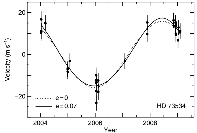
Figure 5. Radial velocities for HD 73534 are fit with an orbital period of 1770 days, velocity amplitude of 16.2 m s ^{-1} , and a nearly circular orbit. Error bars illustrate the quadrature sum of the velocity precision for each measurement and 3.5 m s ^{-1} of jitter (systematic errors and/or intrinsic stellar variability). The assumed stellar mass of 1.23 M_\odot yields M \sin i = 1.10 M_{\text{Jup}} and a semimajor axis of 3.07 AU.
