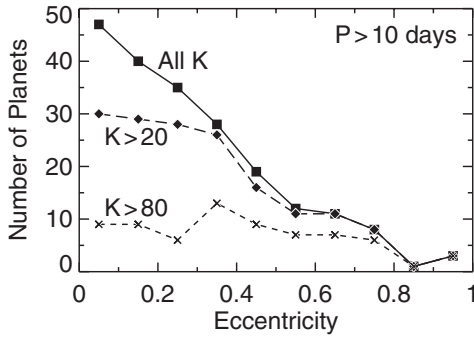
Figure 7. Ignoring planets with periods shorter than 10 days, which may have circularized, the eccentricity distribution for known planets decreases linearly from e = 0 to e = 0.6 . For planets with K > 20 \text{ m s}^{-1} , the distribution is much flatter from e = 0 to e = 0.4 and then declines. For planets with K > 80 \text{ m s}^{-1} , the distribution is flat all the way up to e = 0.8 . These distributions may reflect an observational bias against detecting high-eccentricity planets with velocity semi-amplitudes K near the detection limit, in which case the observed distribution for large K may represent the intrinsic eccentricity distribution for giant planets.
