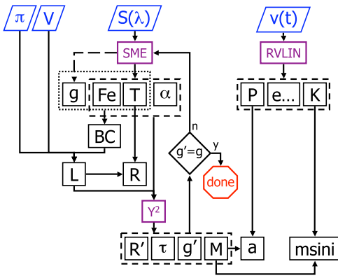
Figure 1. Graphical representation of the analysis flow. Observables in the top row are parallax, apparent visual magnitude, a high-resolution spectrum, and measured radial velocities. The left side shows the spectroscopic (SME) and isochrone ( Y^2 ) analysis, while the right side shows the orbital analysis (RVLIN). Symbols for derived quantities are as described in the text, but with Fe for [Fe/H], \alpha for [\alpha/\text{Fe}] , \tau for age, and g' for g_{\text{iso}} . The arrow pointing up to the g' = g_{\text{iso}} decision diamond illustrates a new outer loop that enforces consistency between spectroscopic and isochrone gravities.
