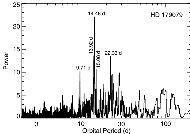
Figure 2. Periodogram of 74 radial velocity measurements for HD 179079. The prominent peak at 14.46 days is consistent with the 14.476 \pm 11 days period returned by a Keplerian fit of the measured velocities. The next four strongest peaks (labeled in the figure) are significantly weaker.
