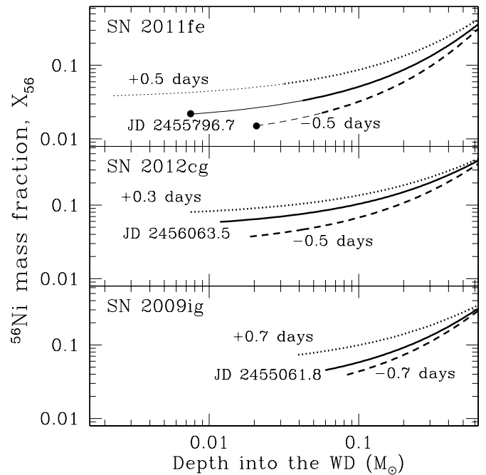
Figure 9. Inferred distribution of ^{56}\text{Ni} as a function of depth in the WD. In each case we compare multiple explosion times, with the solid lines indicating the value preferred by fitting v \propto t^{-0.22} . The depth into the star is assumed to scale as \Delta M_{\text{diff}} \propto t^{1.76} with a normalization of \Delta M_{\text{diff}} = 1.4 M_{\odot} at light curve peak. For SN 2011fe (top panel), the thick curves correspond to the constraints from the observations by Vinkó et al. (2012), and the thin curves correspond to the observations by Nugent et al. (2011). The filled circles indicate the shallowest allowed deposits of ^{56}\text{Ni} so as not to overshoot the upper limit presented by Bloom et al. (2012).
