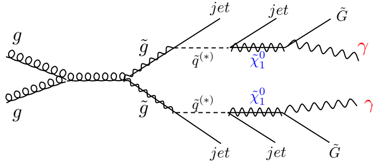
Figure 1: Example diagram of \tilde{\chi}_1^0 pair production and \tilde{\chi}_1^0 \rightarrow \gamma + \tilde{G} decay.
