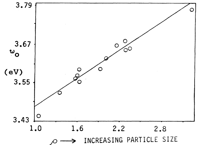
FIG. 2. Plot of the particle-size-dependent function \rho (obtained from the line-shape fit) vs the observed surface-plasmon resonance frequency. The straight line has the function 0.147\rho + 3.325 = \gamma(\text{eV}) . The correlation coefficient for the linear regression is 0.97. The data indicate a red shift of the surface-plasmon resonance with decreasing particle size, in contrast to a blue shift observed for matrix-supported silver particles.
